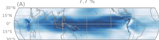
Zonal Winds at 850 hPa
