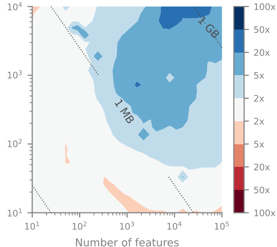
B | Speed-up xeofs vs. eofs
