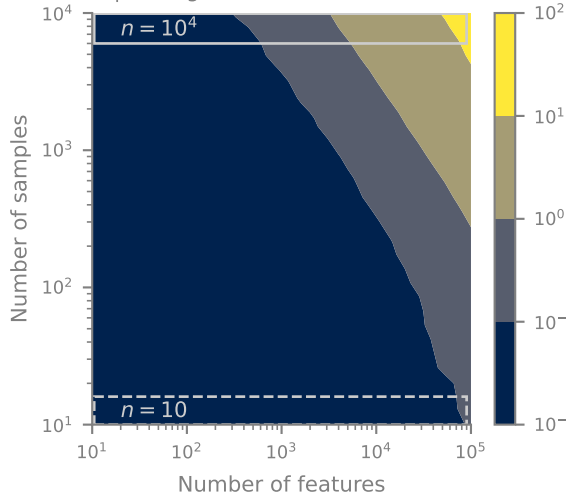
A | Timings of xeofs [in s]
