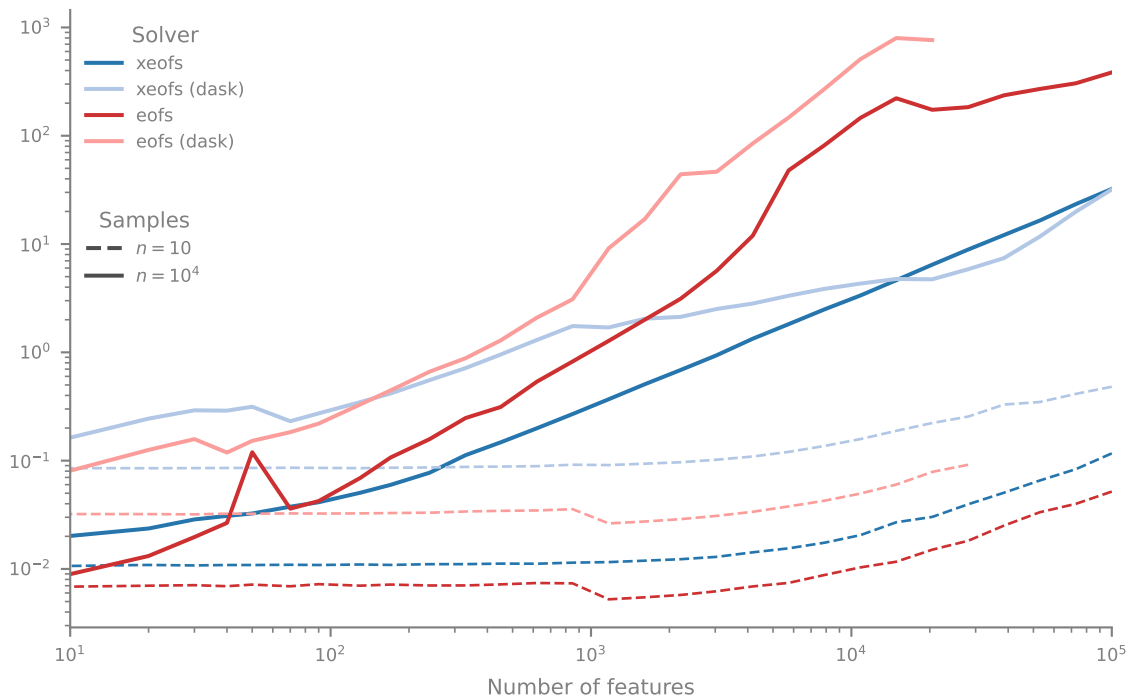
C | Timings vs. number of features [in s]
