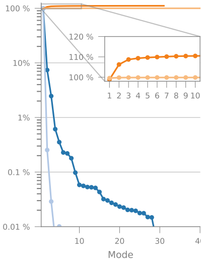
A | Squared Covariance Fraction (SCF)
