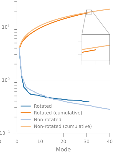
C | Squared Singular Values \sigma^2
