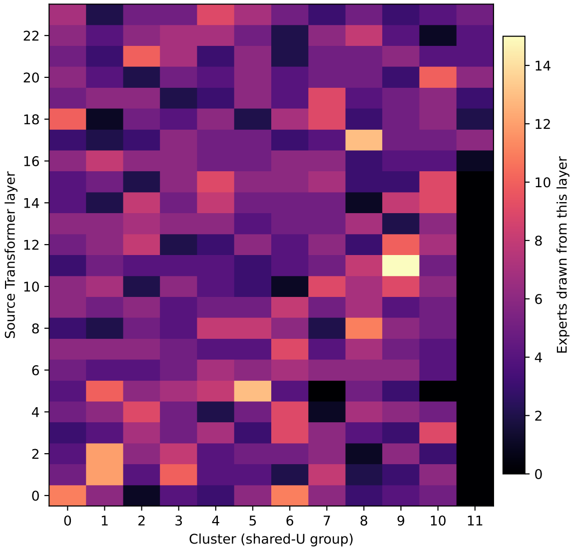
Layer x cluster composition — down_proj (Qwen1.5-MoE: 24 layers x 60 experts, 12 groups)
