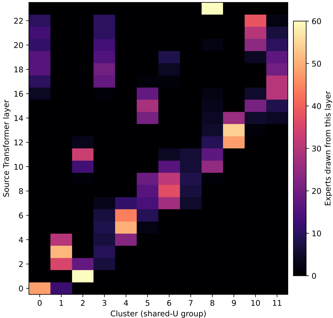
Layer \times cluster composition — gate_proj (Qwen1.5-MoE: 24 layers \times 60 experts, 12 groups)
