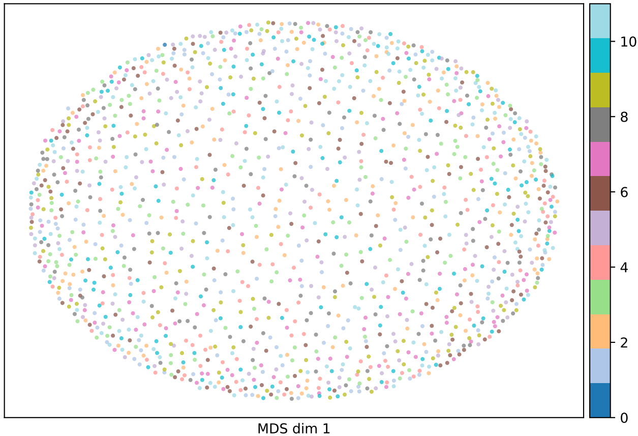
2D MDS of expert subspaces — down_proj (color = shared-U cluster; same color together = coherent)
