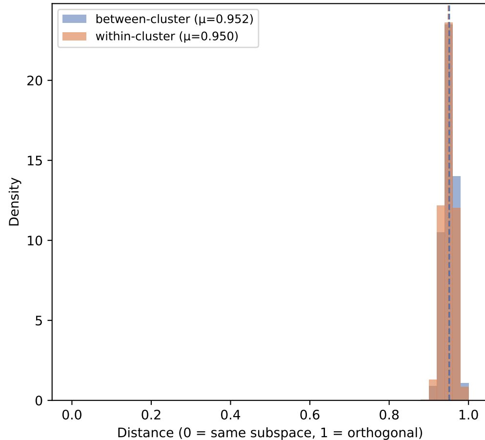
Pairwise Grassmannian distance — down_proj
