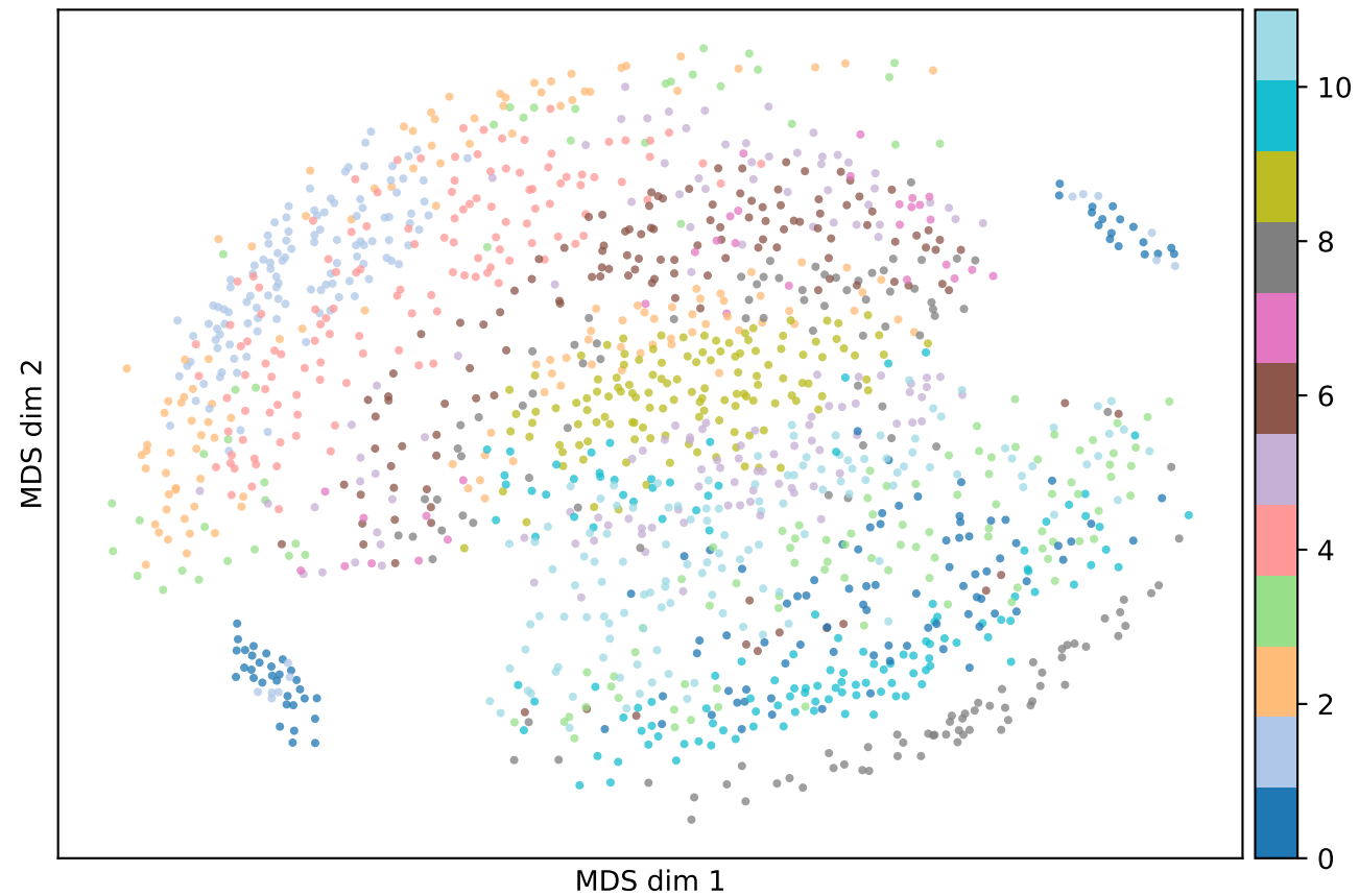
2D MDS of expert subspaces — gate_proj (color = shared-U cluster; same color together = coherent)
