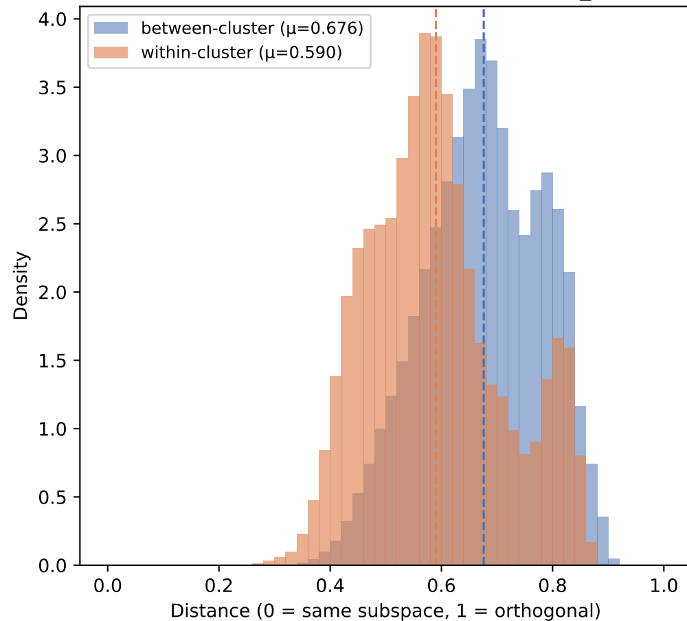
Pairwise Grassmannian distance — gate_proj
