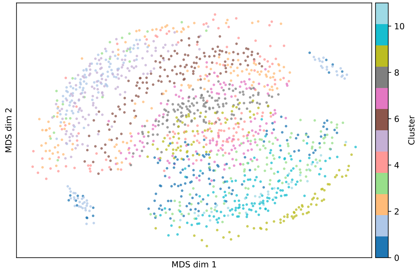
2D MDS of expert subspaces — up_proj (color = shared-U cluster; same color together = coherent)
