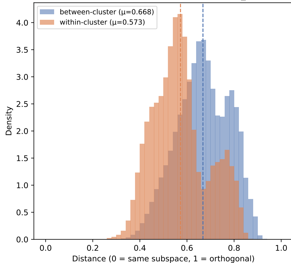
Pairwise Grassmannian distance — up_proj
