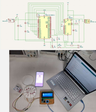
Pill Dispenser (Hardware)
