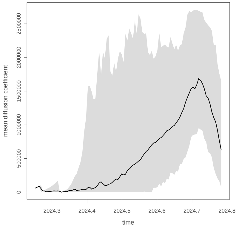
Evolution of mean diffusion coefficient
