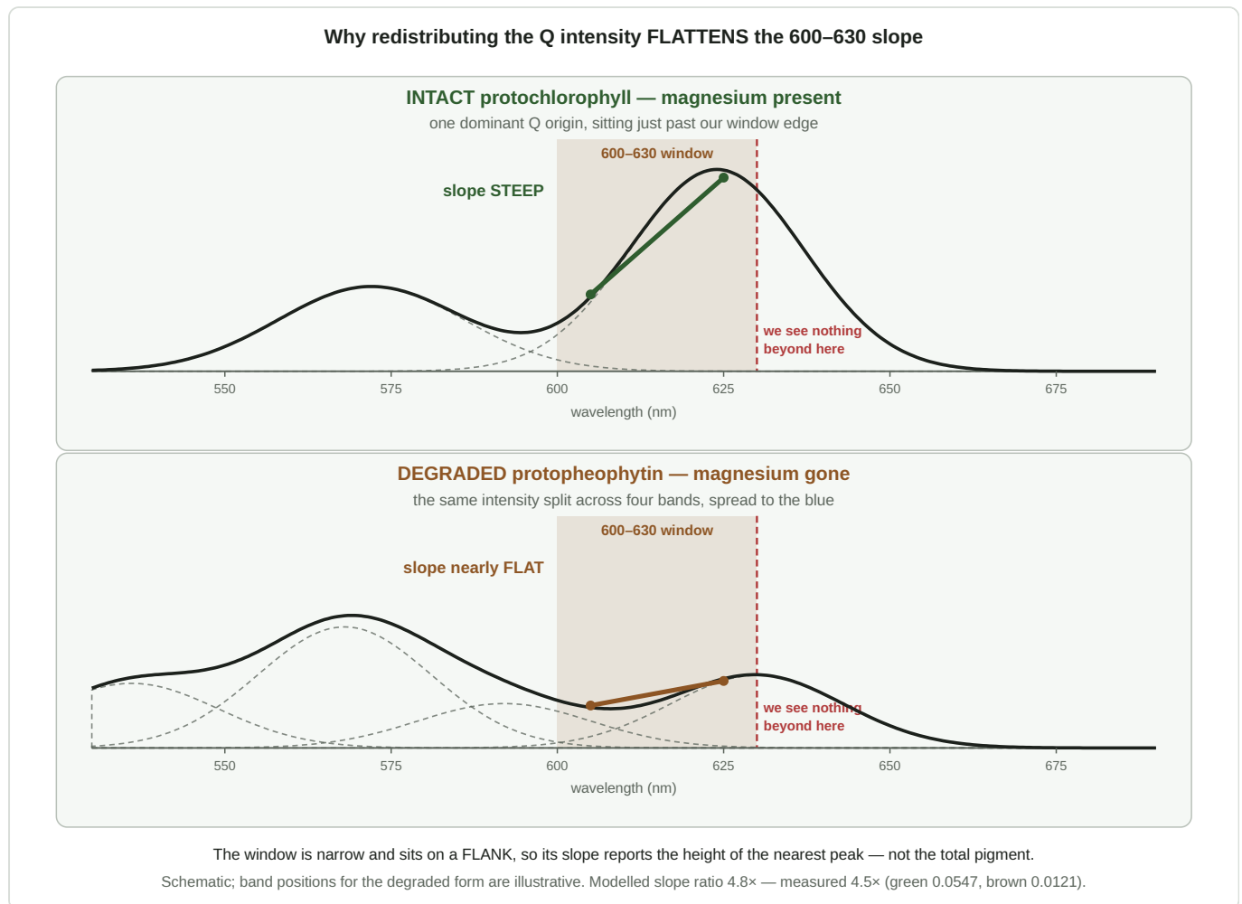
Figure 4 — the mechanism. Top: with the magnesium intact, one dominant Q origin sits just past our capture limit, and its rising flank sweeps straight through the 600–630 window — so the absorbance climbs steeply across it. Bottom: once the magnesium is gone, that same intensity is spread across several weaker bands further to the blue. Nothing tall is left near 630, the window now lies on a shallow shoulder, and the slope across it nearly vanishes. The total area under the two curves is similar; only its distribution differs. Schematic — the degraded band positions are illustrative — but the modelled slope ratio (4.8×) is close to the measured one (4.5×).
