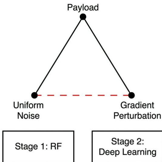
Figure 22: The Defense Structures
