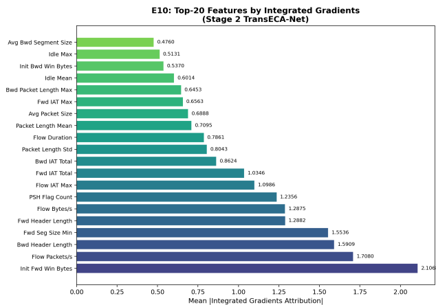
Figure 9: Global Integrated Gradients
