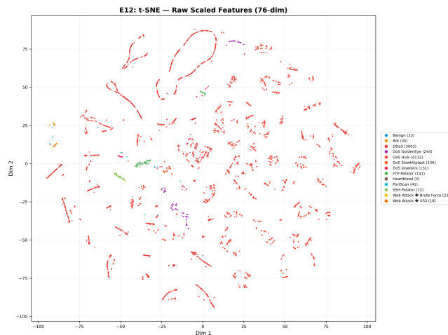
Figure 20: Topological Entanglement in Raw Feature Space
