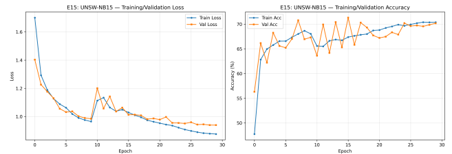
Figure 4: Training Evolution
