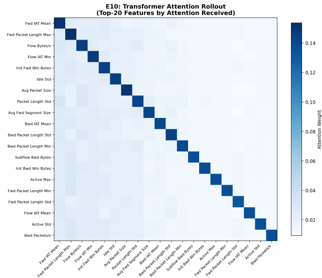
Figure 11: Attention Heatmap
