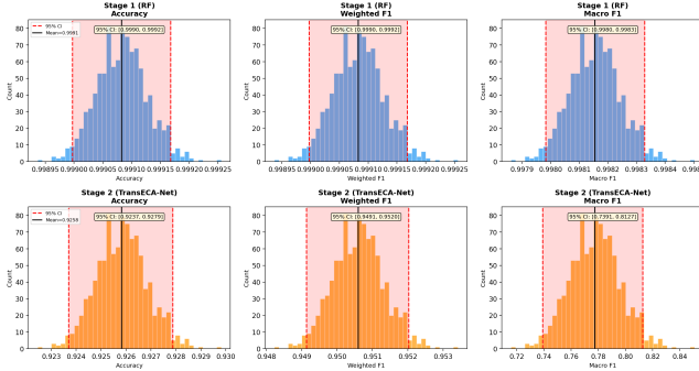
Figure 13: Statistical Boundaries
