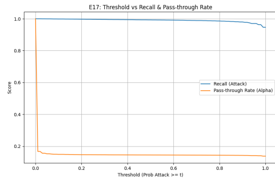
Figure 1: Threshold Tuning
