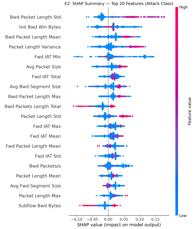
Figure 7: SHAP Attribution
