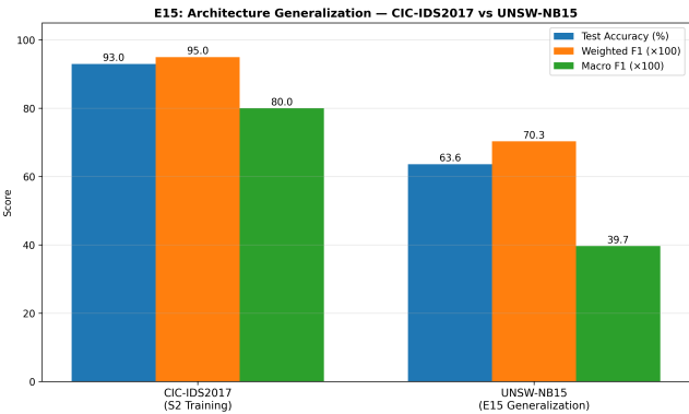
Figure 6: Cross-Dataset Degradation
