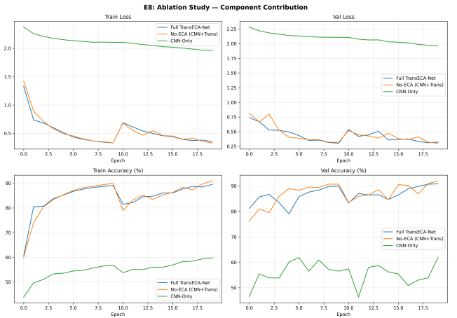
Figure 2: Architecture Ablation
