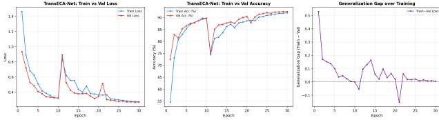
Figure 17: Generalization Gaps
