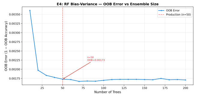
Figure 16: OOB Convergence Bounds
