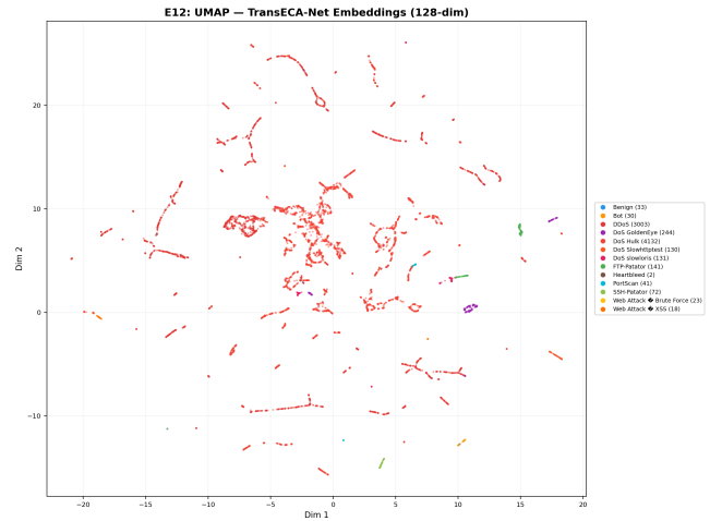
Figure 19: Deep Representational Reconstruction and Cluster Evolution (UMAP)
