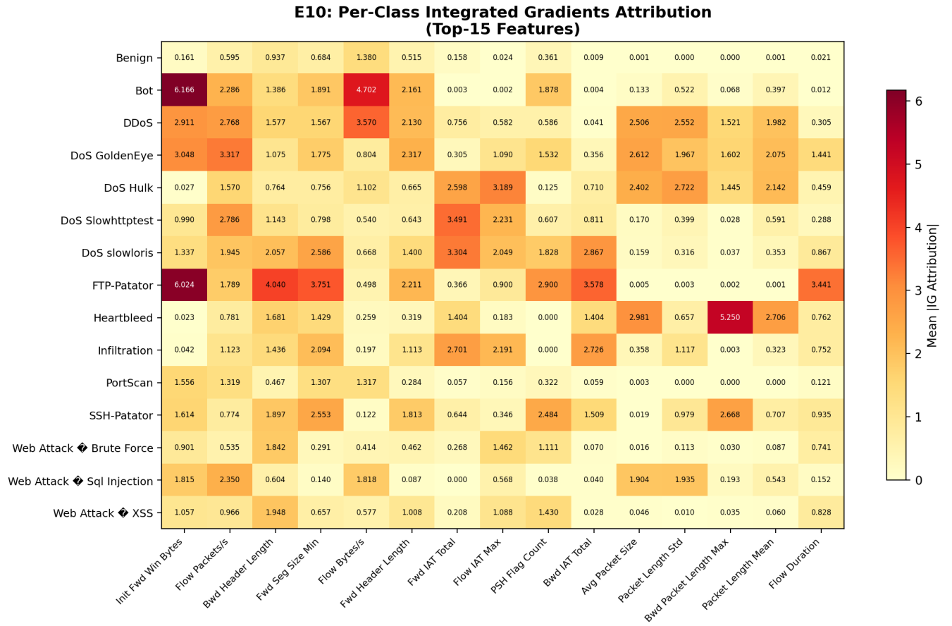
Figure 10: Per-Class Topological Isolation (IG Heatmap)
