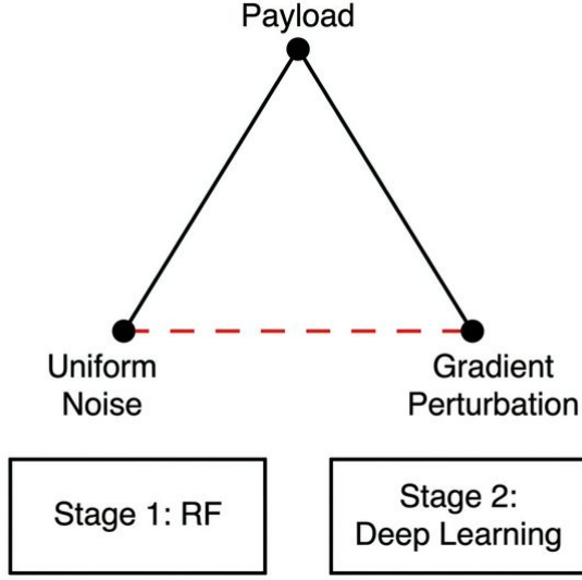
Figure 20: The Defense Structures (Impossible Trinity)
