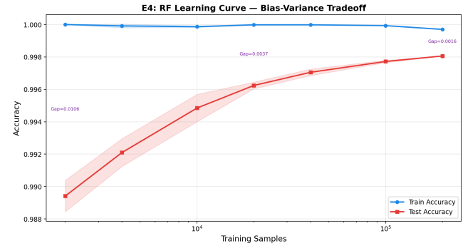
Figure 17: Data Saturation Effect (RF Learning Curve)
