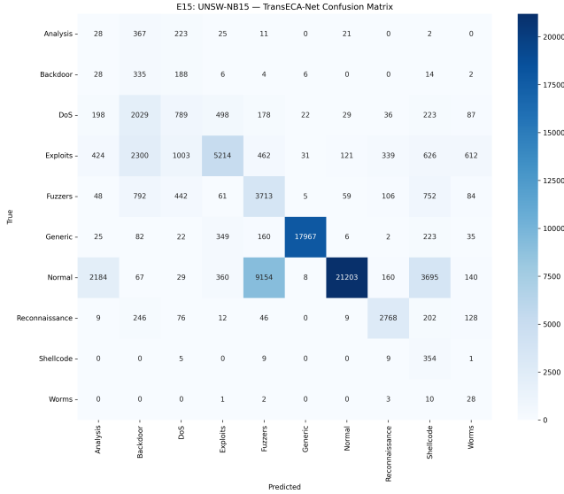
Figure 5: Cross-Dataset Confusion Matrix (UNSW-NB15)
