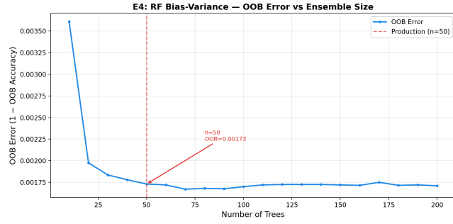
Figure 14: OOB Convergence Bounds
