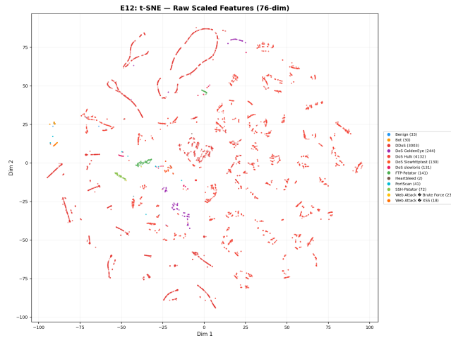
Figure 18: Topological Entanglement in Raw Feature Space (t-SNE)
