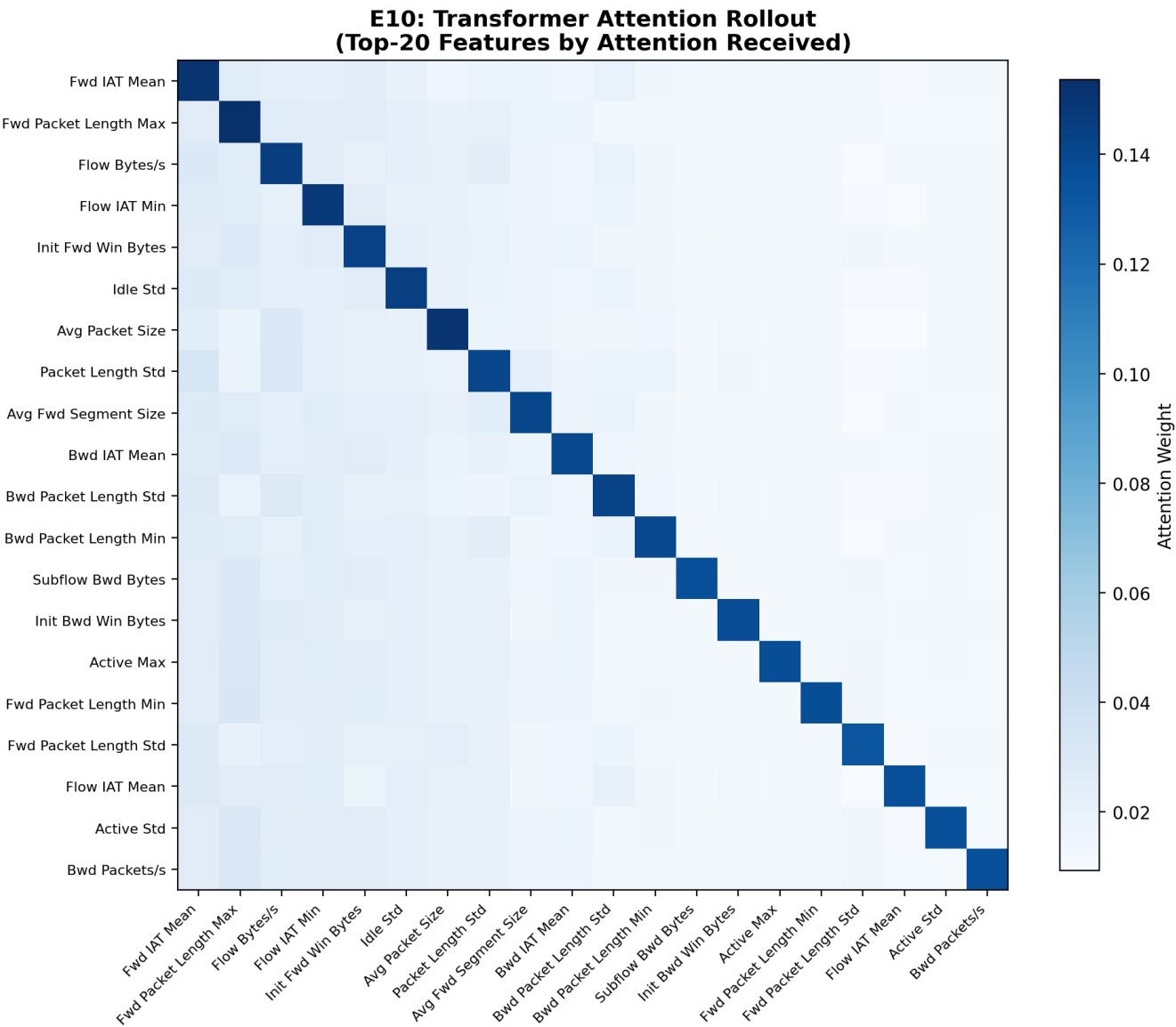
Figure 11: Transformer Attention Heatmap
