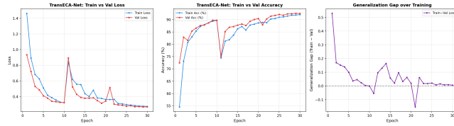
Figure 15: Generalization Gaps (DL Learning Curves)
