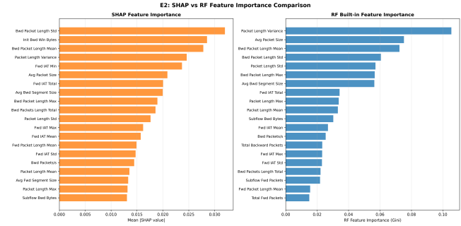
Figure 8: Axiomatic Consistency (SHAP vs. RF Gini)
