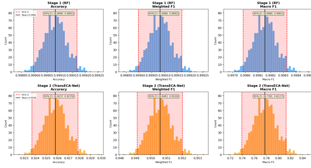
Figure 13: Statistical Boundaries (Bootstrap Distributions)
