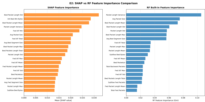
Figure 8: Axiomatic Consistency
