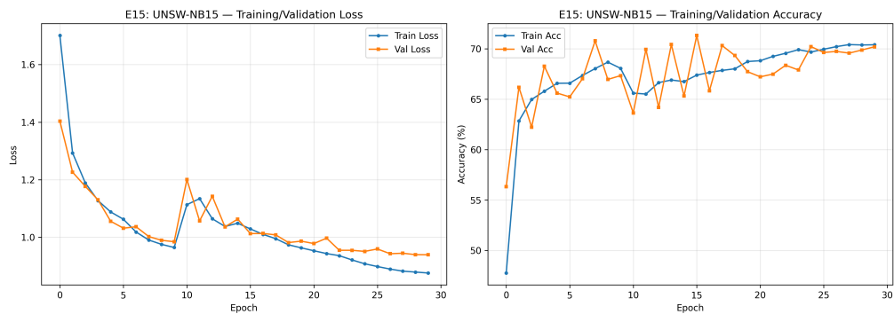
Figure 4: Training Evolution
