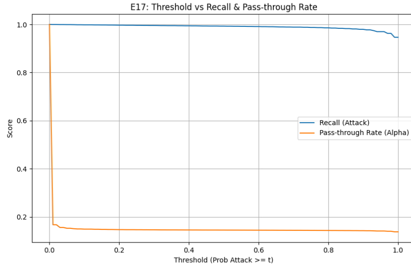
Figure 1: Threshold Tuning
