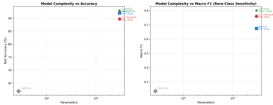
Figure 18: Capacity Topographic Jump
