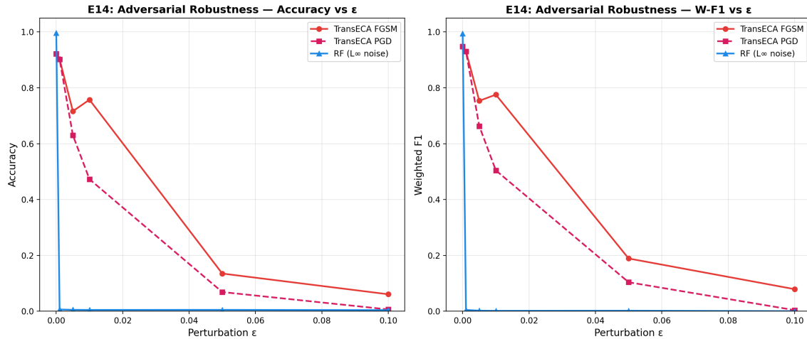
Figure 14: Attack Resilience Curves
