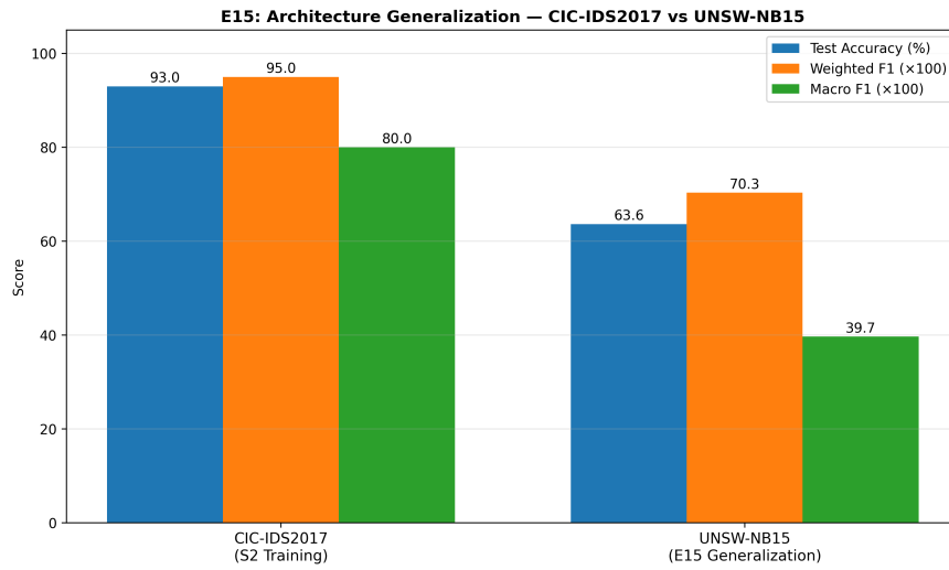
Figure 6: Cross-Dataset Degradation
