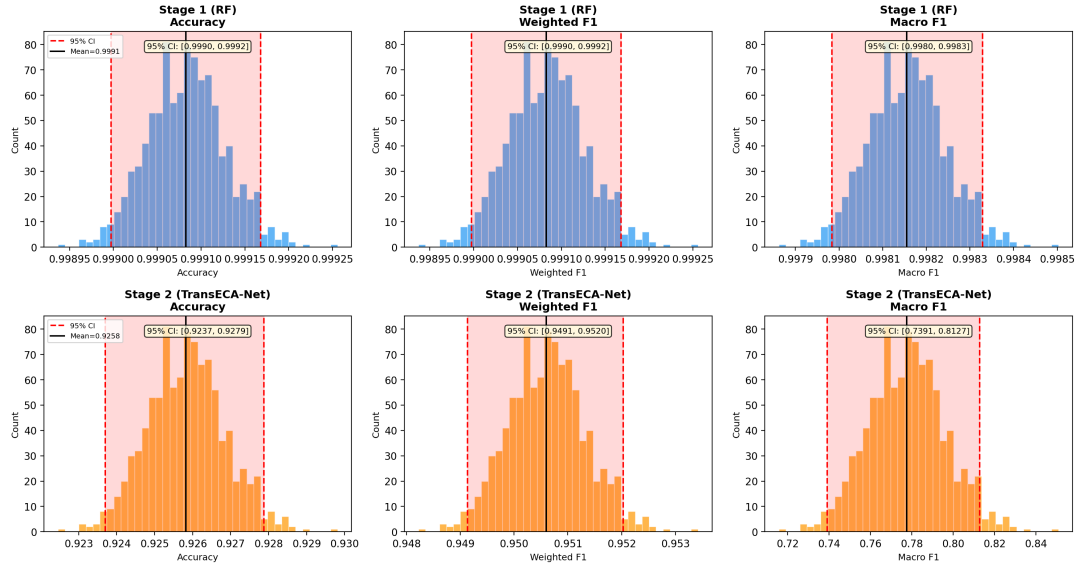
Figure 13: Statistical Boundaries
