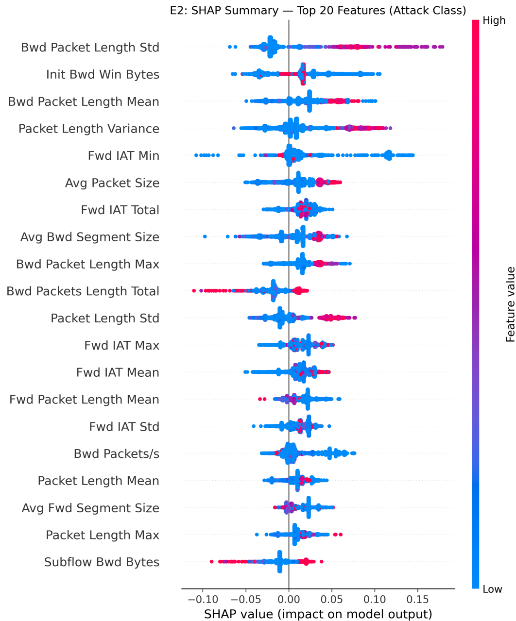
Figure 7: SHAP Attribution
