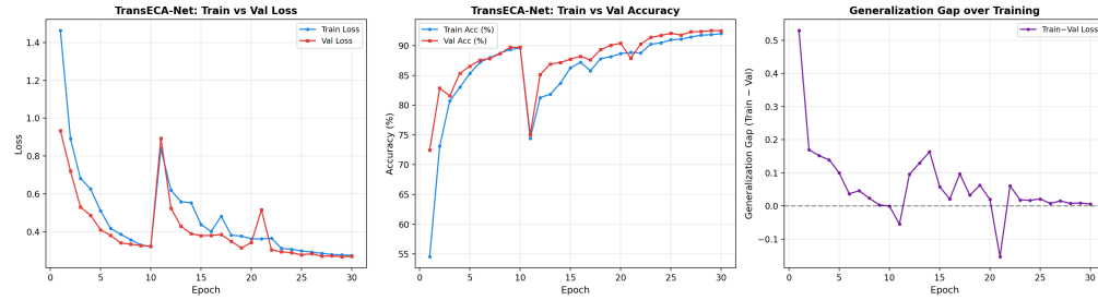
Figure 17: Generalization Gaps
