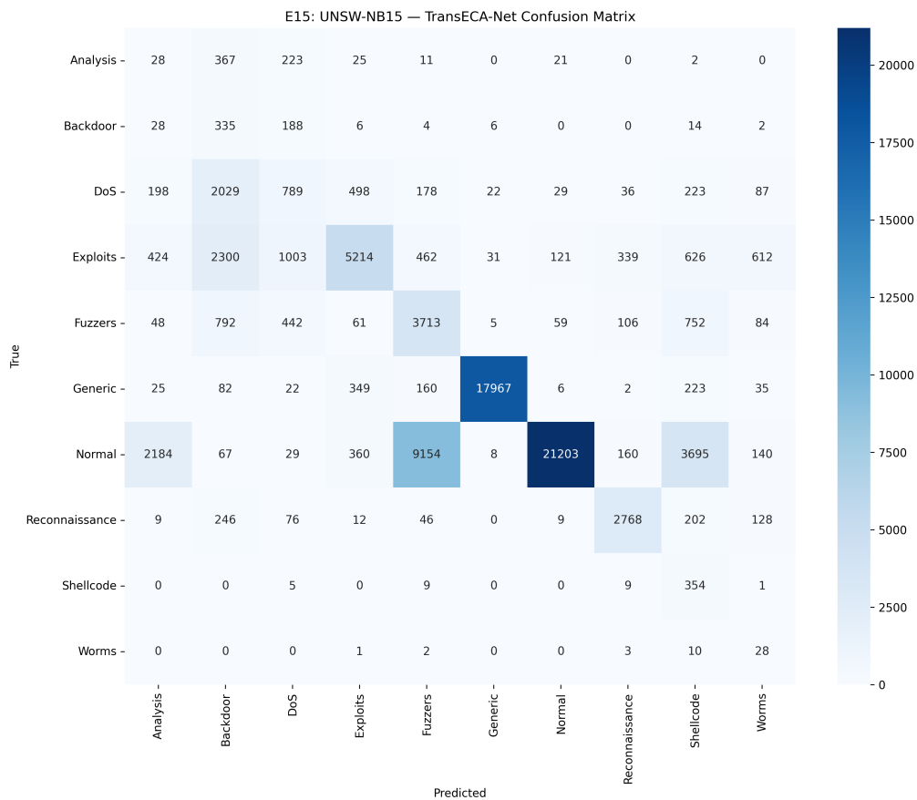
Figure 5: Confusion Matrix
