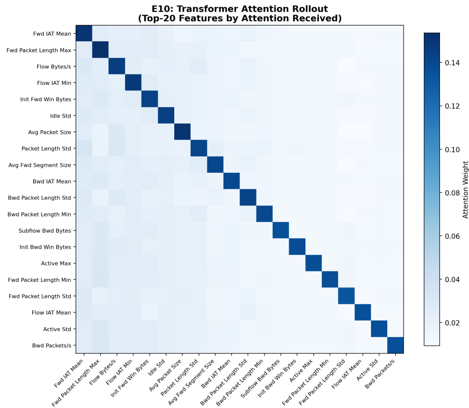
Figure 11: Attention Heatmap
