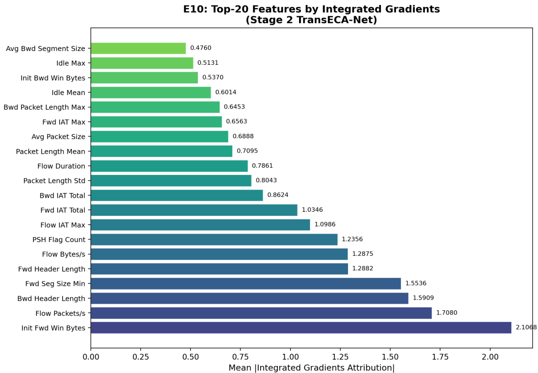
Figure 9: Global Integrated Gradients
