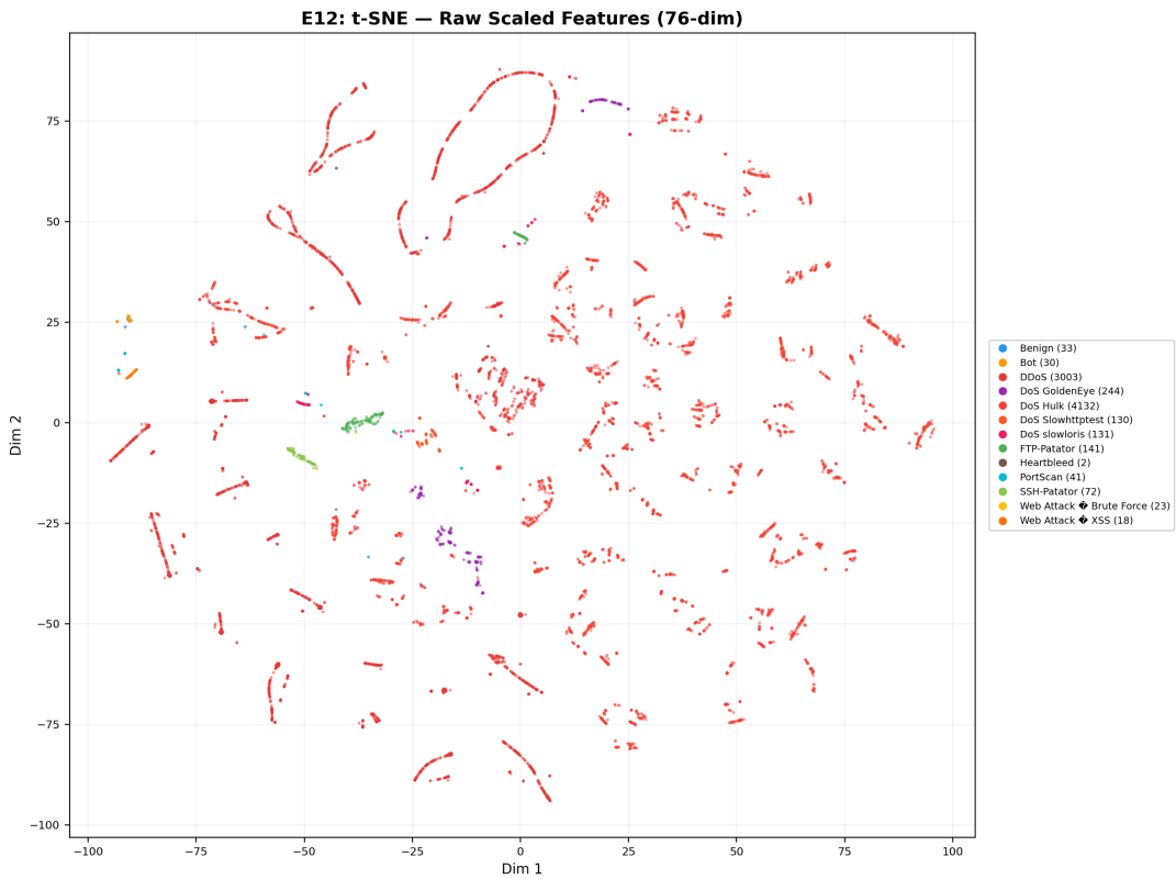
Figure 20: Topological Entanglement in Raw Feature Space
