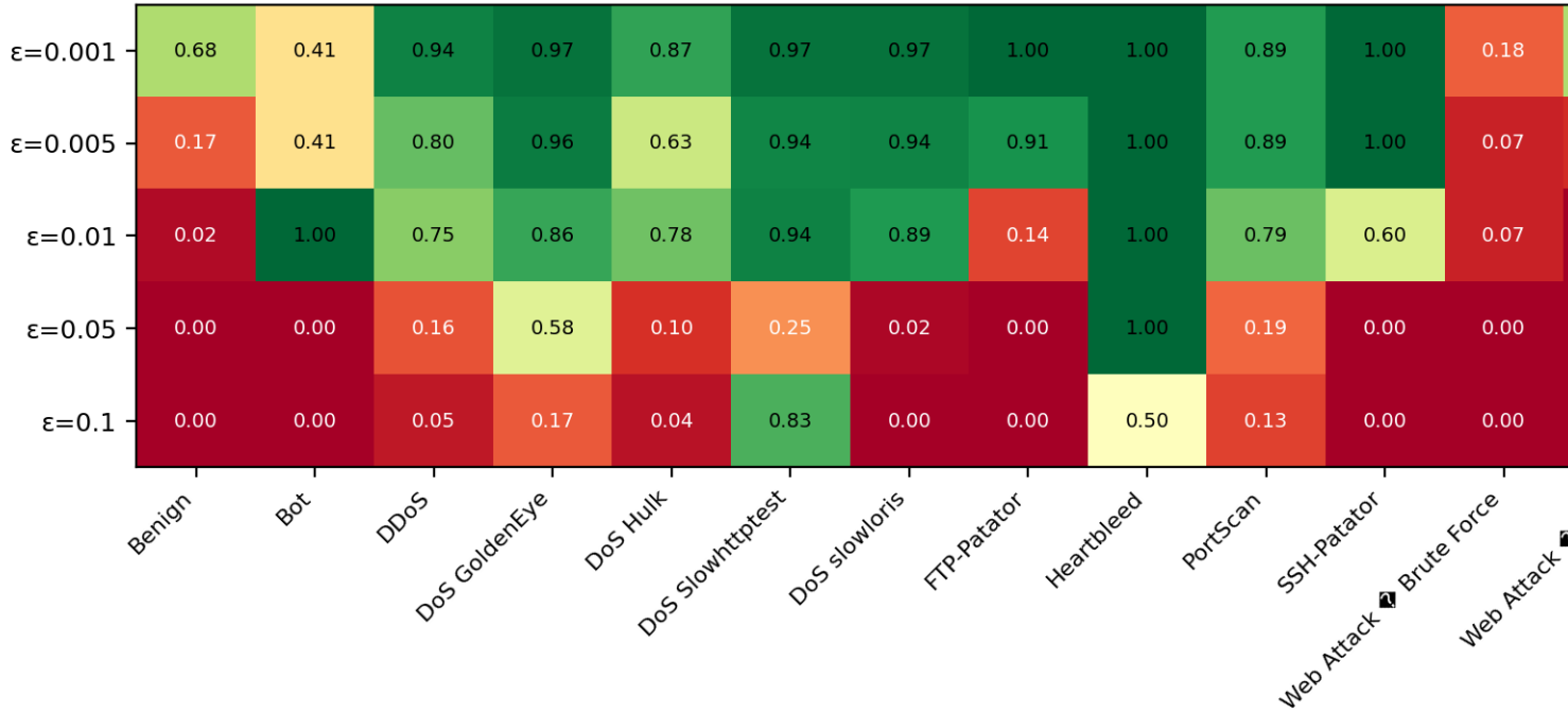
Figure 15: Class Penetration Rates and Adversarial Priority
