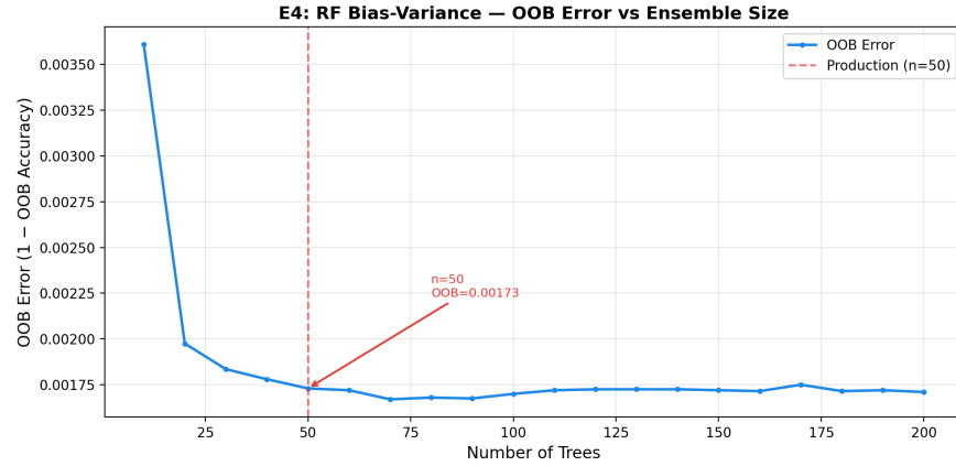
Figure 16: OOB Convergence Bounds
