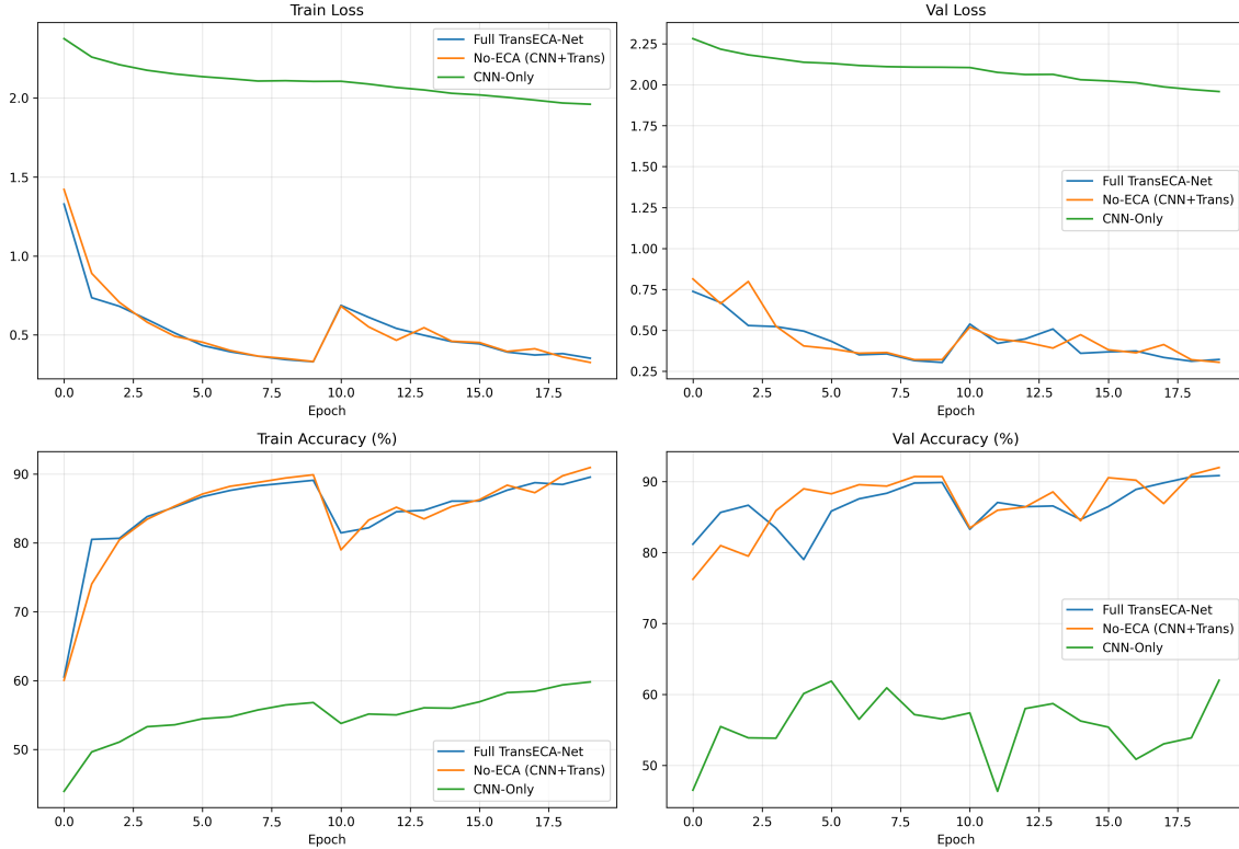
E8: Ablation Study — Component Contribution
