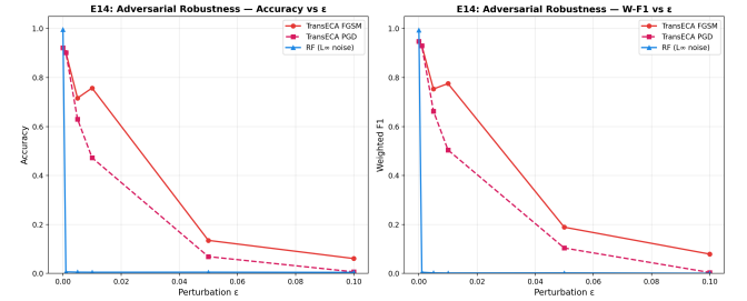
Figure 14: Attack Resilience Curves
