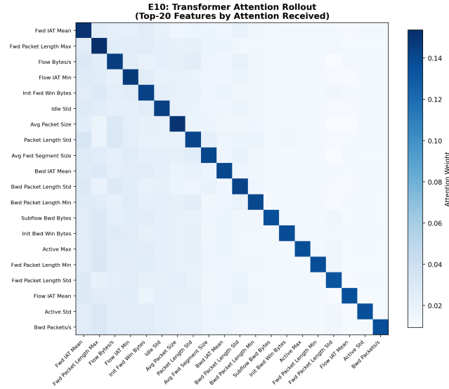
Figure 11: Attention Heatmap
