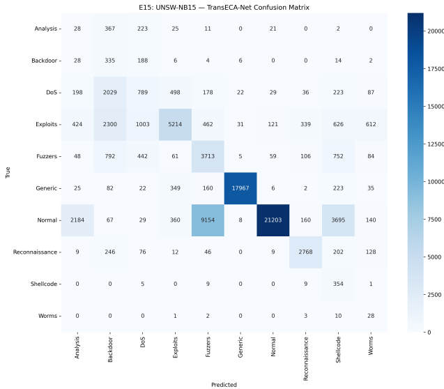
Figure 5: Confusion Matrix
