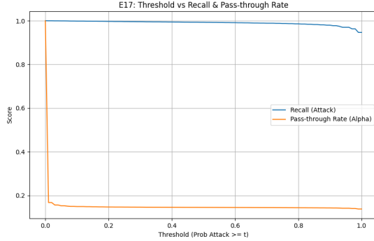
Figure 1: Threshold Tuning
