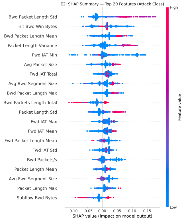
Figure 7: SHAP Attribution
