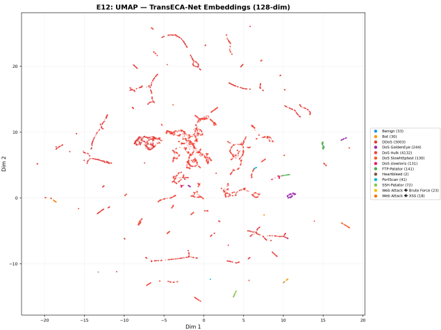
Figure 21: Deep Representational Reconstruction and Cluster Evolution
