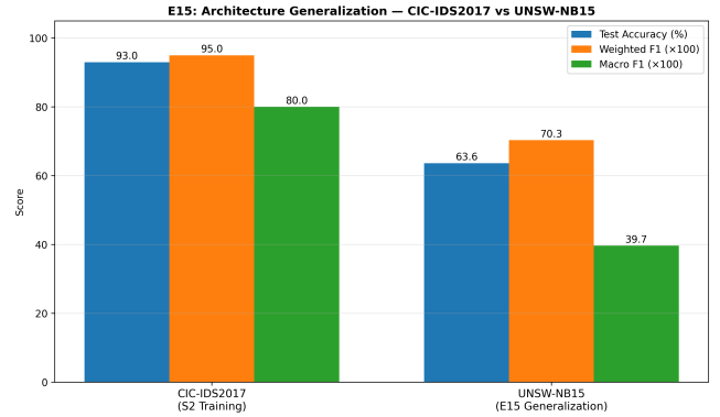
Figure 6: Cross-Dataset Degradation
