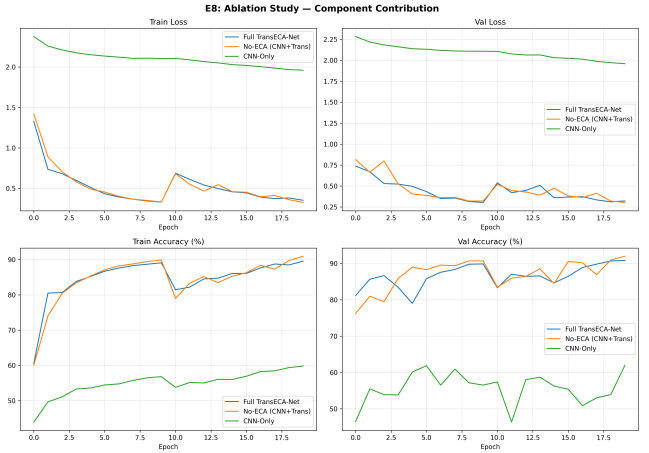
Figure 2: Architecture Ablation
