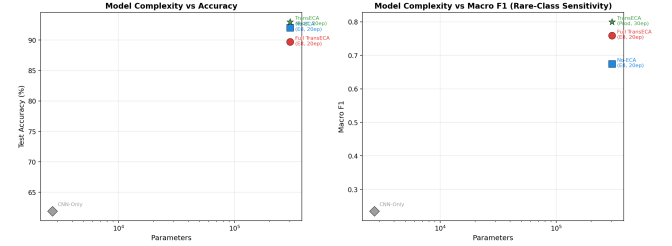
Figure 18: Capacity Topographic Jump
