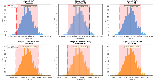
Figure 13: Statistical Boundaries
