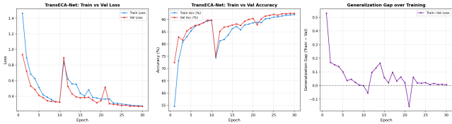
Figure 17: Generalization Gaps
