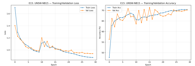
Figure 4: Training Evolution
