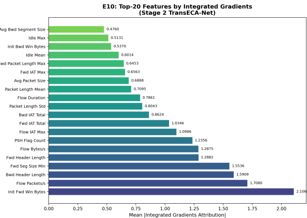
Figure 9: Global Integrated Gradients
