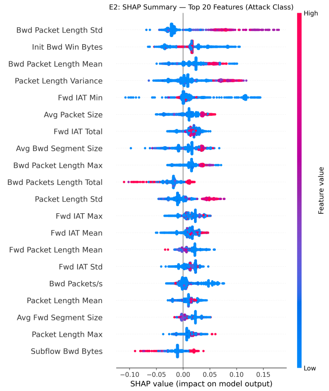
Figure 7: SHAP Attribution
