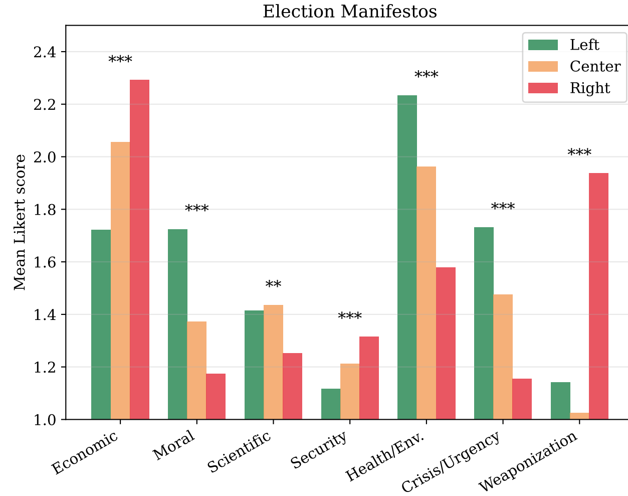
Frame Scores by Ideological Bloc (* p<0.05, ** p<0.01, *** p<0.001)
