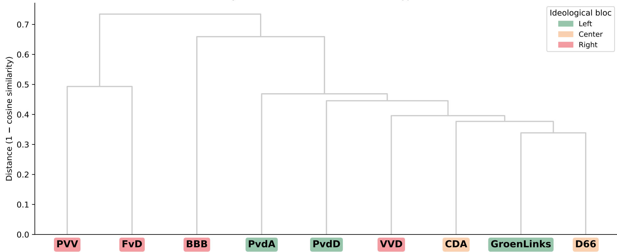
Hierarchical Clustering of Parties by Lexical Similarity (Ward linkage, cosine distance on TF-IDF, all text types combined)
