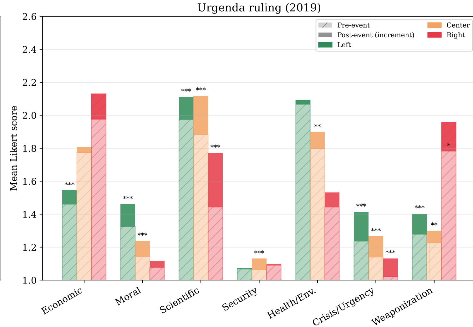
Frame Scores Before and After Shock Events by Ideological Bloc Hatched bars show pre-event mean; solid increment shows post-event change (* p<0.05, ** p<0.01, *** p<0.001)
