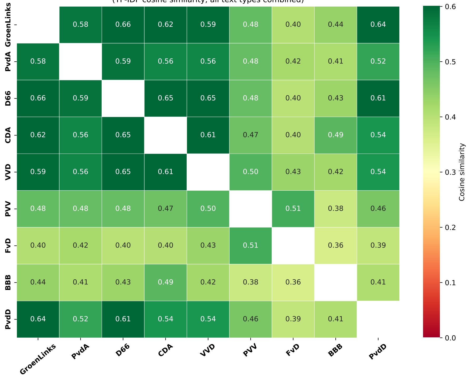
Lexical Similarity Between Parties in Climate Discourse (TF-IDF cosine similarity, all text types combined)
