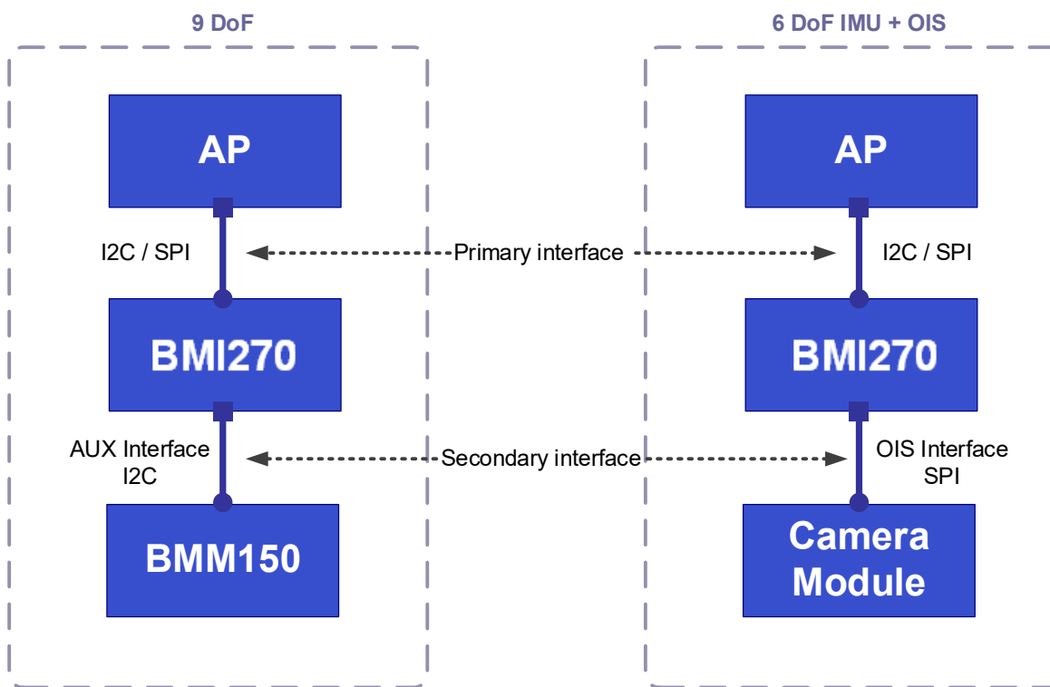
Figure 9: Digital Interfaces
