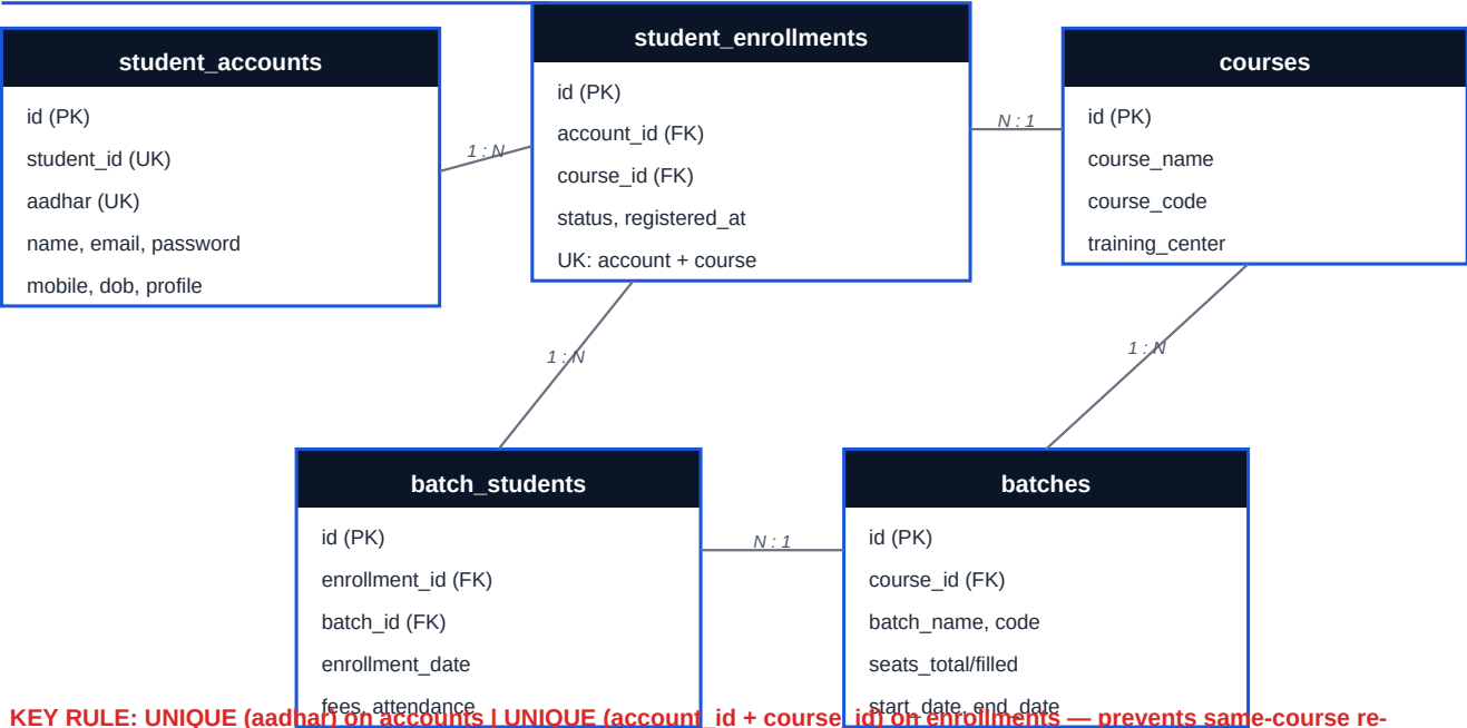
Diagram 2 — Database Structure (ER Diagram)
