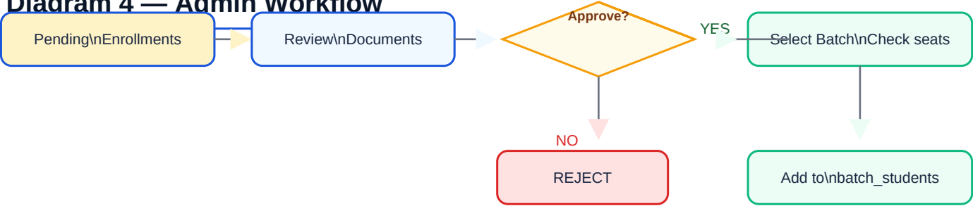
Diagram 4 — Admin Workflow
