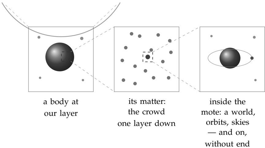
Figure 4.2.: Layers inside layers. The layers are not side by side; they are inside one another. A body at our layer (left), magnified, is a crowd of motes — the layer below, which constitutes our matter and our “empty” space alike (middle). Open any mote and there is structure again: bodies, orbits, room for skies (right) — and so on, without end, in both directions: the dashed lines above the first frame continue outward, because everything shown is itself one mote in a body at the layer above. Scale is invisible from within; every frame’s inhabitants measure themselves person-sized and their moment as now, and each is correct.
