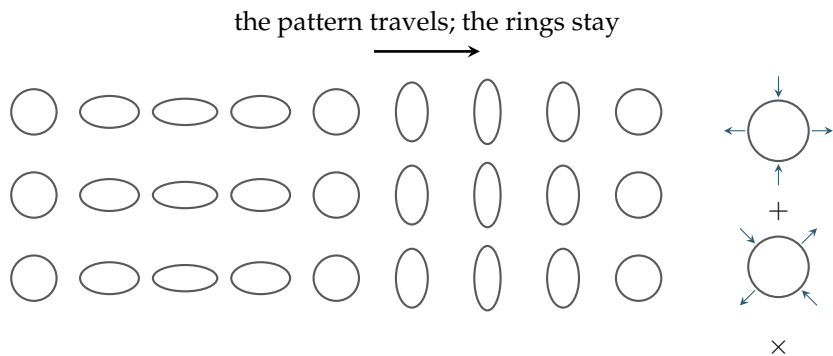
Figure 7.3.: What the wave does. A lattice of rings of free test particles; each column is caught at a slightly later beat of the same kneading pulse, so a sinusoid made of shapes stands written across the grid — and the whole pattern slides through at the speed of light while the rings stay where they are, a stadium wave crossing a crowd that never leaves its seats. Right: the two flavours of the breathing — stretch along the axes (plus) or along the diagonals (cross). Between them lies everything a gravitational wave can do.
