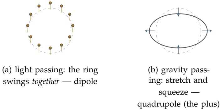
Figure 7.4.: The two songs have different shapes. A ring of test particles under a passing light wave (a) swings back and forth as one — both of light’s polarizations are of this dipole kind, one per axis. Under a passing gravitational wave (b) the same ring is kneaded — stretched one way, squeezed the other — in the quadrupole plus and cross of the ring lattice. One medium carrying both means one crowd with exactly these two transverse branches, at one speed, and no others: the sharpened second problem of the research program.
