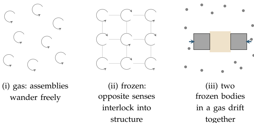
Figure 6.5.: States of the crowd. (i) Gas: assemblies wander, all agitation and passage. (ii) Frozen: neighbouring circulations of opposite sense interlock into a structure that holds its shape — matter as local winter; heat the crowd past what the interlocking can absorb and the structure lets go, which is what decay is. (iii) Two frozen bodies in a gas shelter each other: the agitation between them (shaded) is calmer than the agitation outside, and the outside wins — the shadow push reappearing at a new scale, unbidden.
