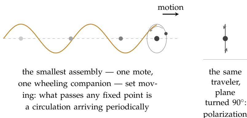
Figure 6.6.: The first sketch of light: an object orbited by another, in motion — a particle doing a wave. The traveling pair is as localized as any particle and delivers its pushes in discrete arrivals; the pattern of those arrivals along the path is as periodic as any wave, with a frequency (the wheeling rate) and an orientation (the plane of the orbit). Turn the plane ninety degrees (right) and you have the other polarization — not a property bolted on, but geometry the object could not help having. The section keeps this picture — demoted: as the portrait of a localized wave-packet of the medium, not the traveler itself.
