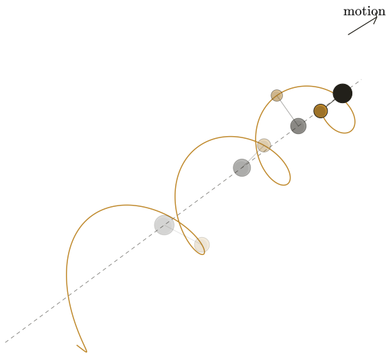
the same traveler, plane turned 90°: polarization
