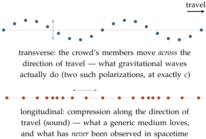
Figure 7.5.: The specification nature hands the layer below. If “space waving” is really the crowd below in motion, the crowd is not generic: its waves must be transverse only (top), in exactly two polarizations, at exactly the speed of light — and it must carry no longitudinal, sound-like mode (bottom), though ordinary media love nothing better. Add the Michelson–Morley demand that the crowd’s rest frame never show itself, and the reply to the gravitational-wave objection survives only as a very special crowd indeed.
