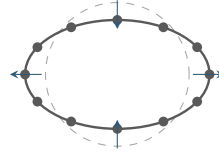
(b) gravity passing: stretch and squeeze — quadrupole (the plus)
