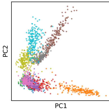
Fixed random
