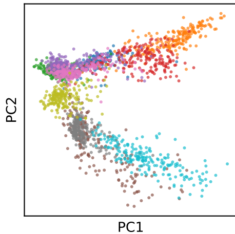
Hard-to-easy
