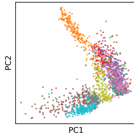
Easy-to-hard
