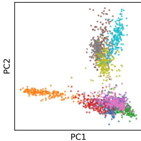
Random reshuffle
