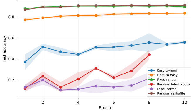
(a) Test accuracy over training. The random and fixed-random runs converge fastest, while class-ordered streams fail under the default learning rate.
