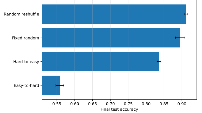
(a) Final test accuracy, averaged over seeds. Error bars denote standard deviation.
