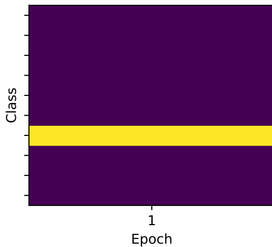
Label sorted
