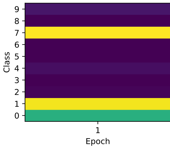
Hard-to-easy
