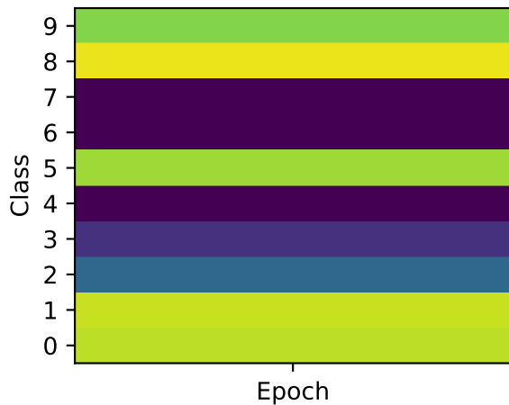
Hard-to-easy
