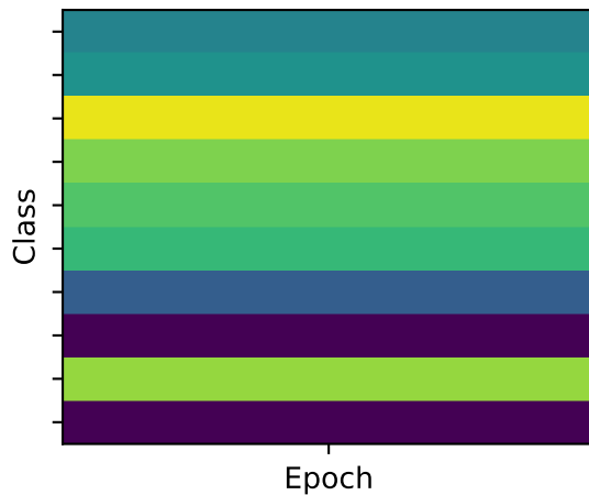
Label sorted
