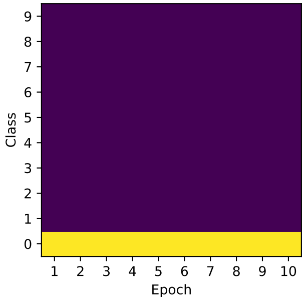
Label sorted
