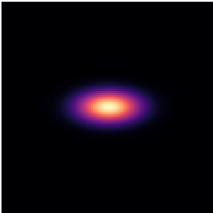
Intrinsic
