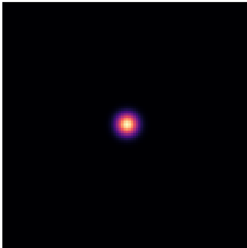
PSF
