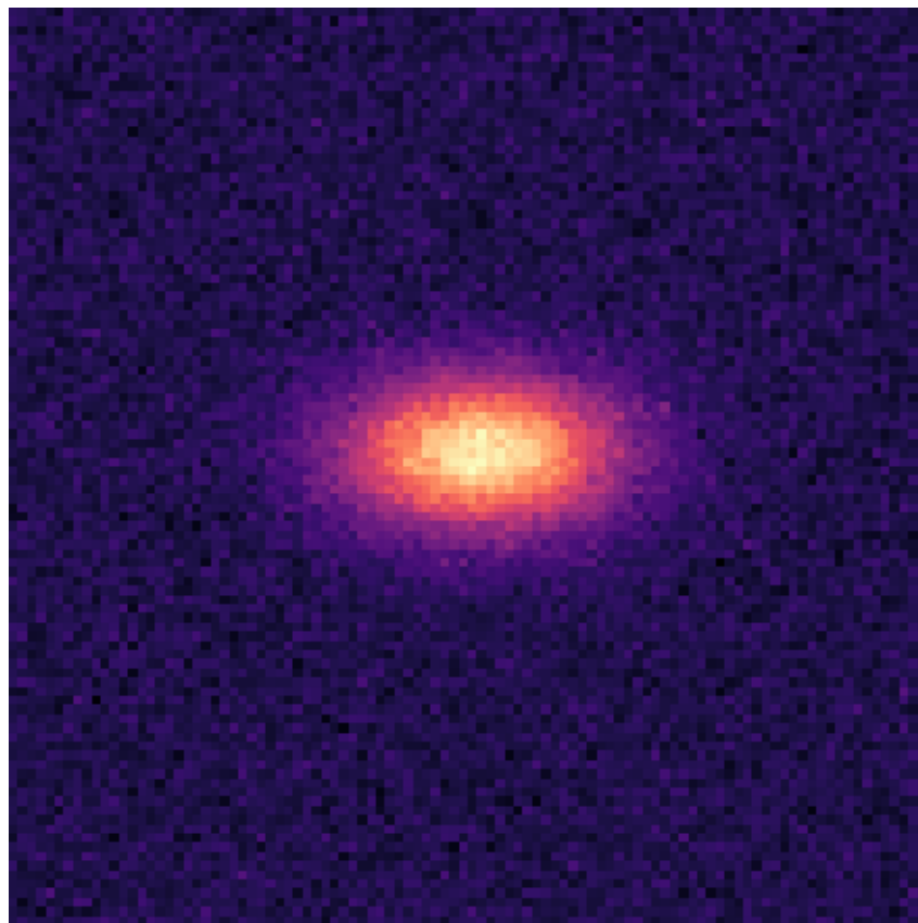
Observed
