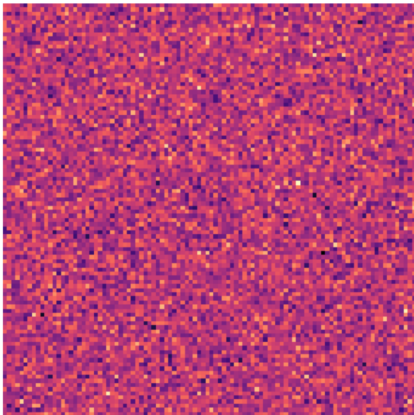
Noise
