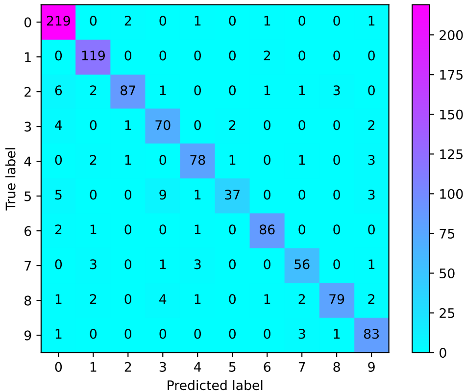
KNN Test Set
