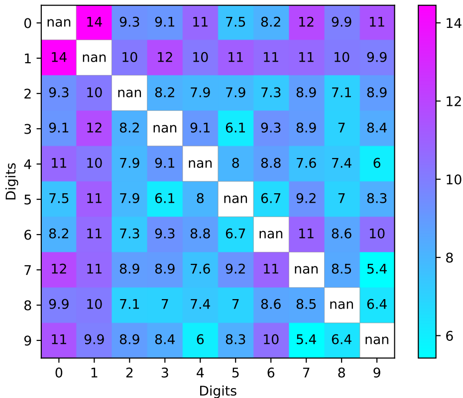
Distance Matrix
