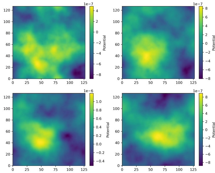
Figure 10: Potential computed using the FFT method for different slices.
