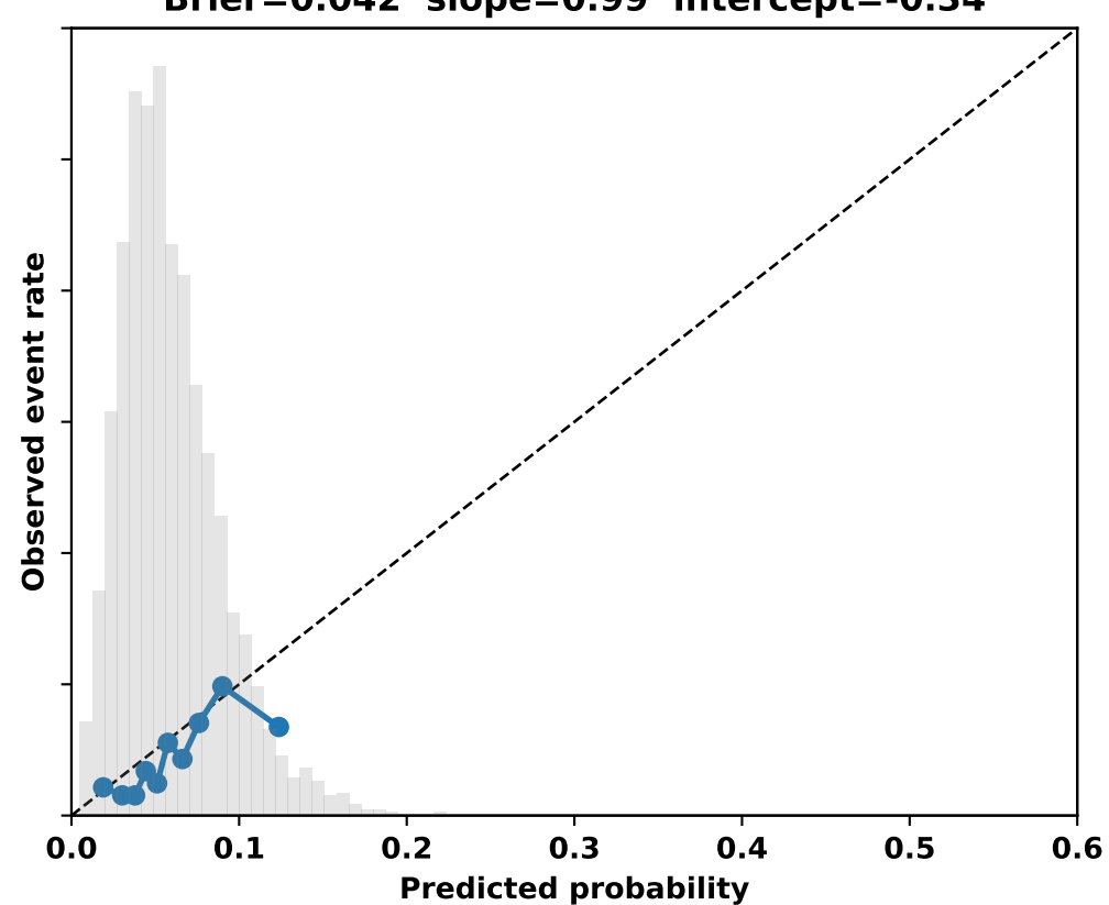
eICU pure Set C (no prior sz/AED/MV) Brier=0.042 slope=0.99 intercept=-0.34
