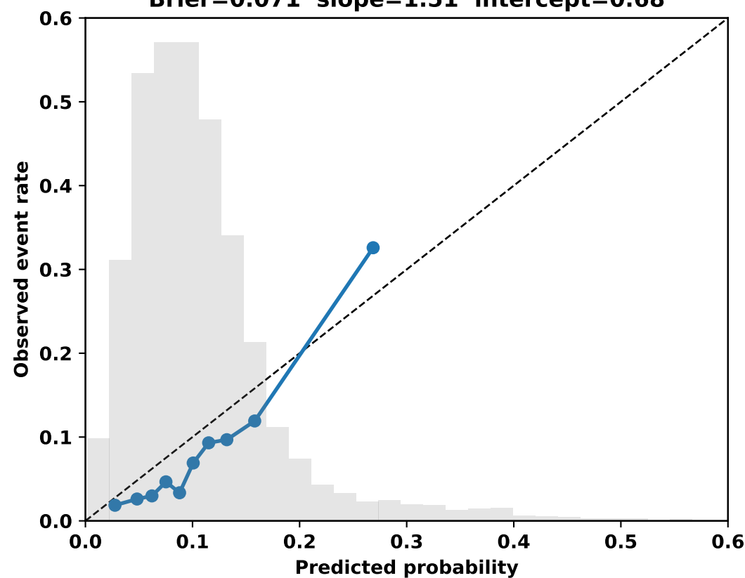
eICU Set C (103 features) Brier=0.071 slope=1.51 intercept=0.68
