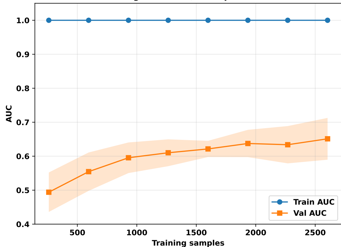
Learning curve (RF, eICU pure Set C)
