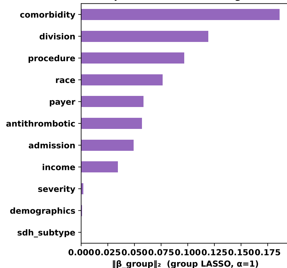
Group-level coefficient magnitudes
