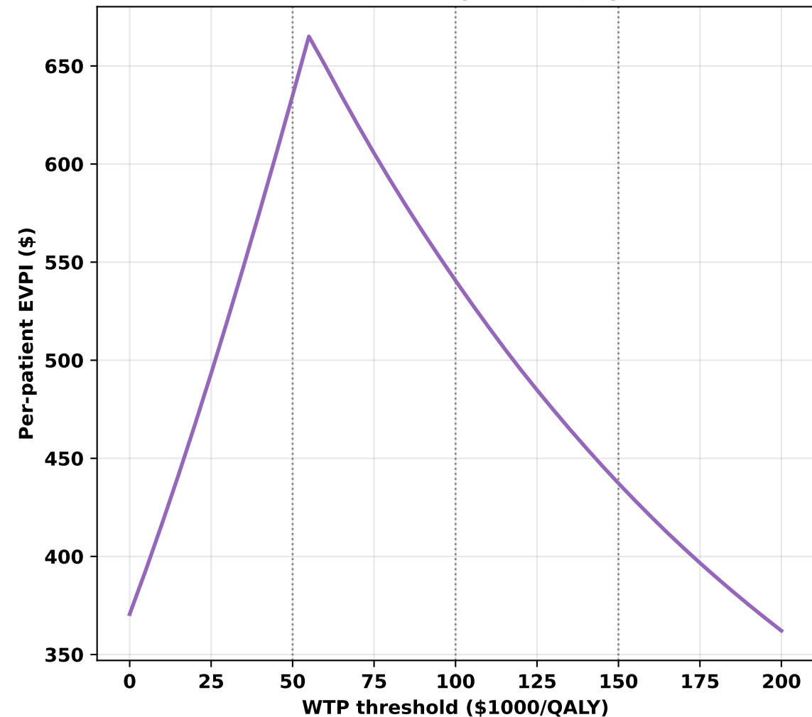
EVPI vs willingness-to-pay
