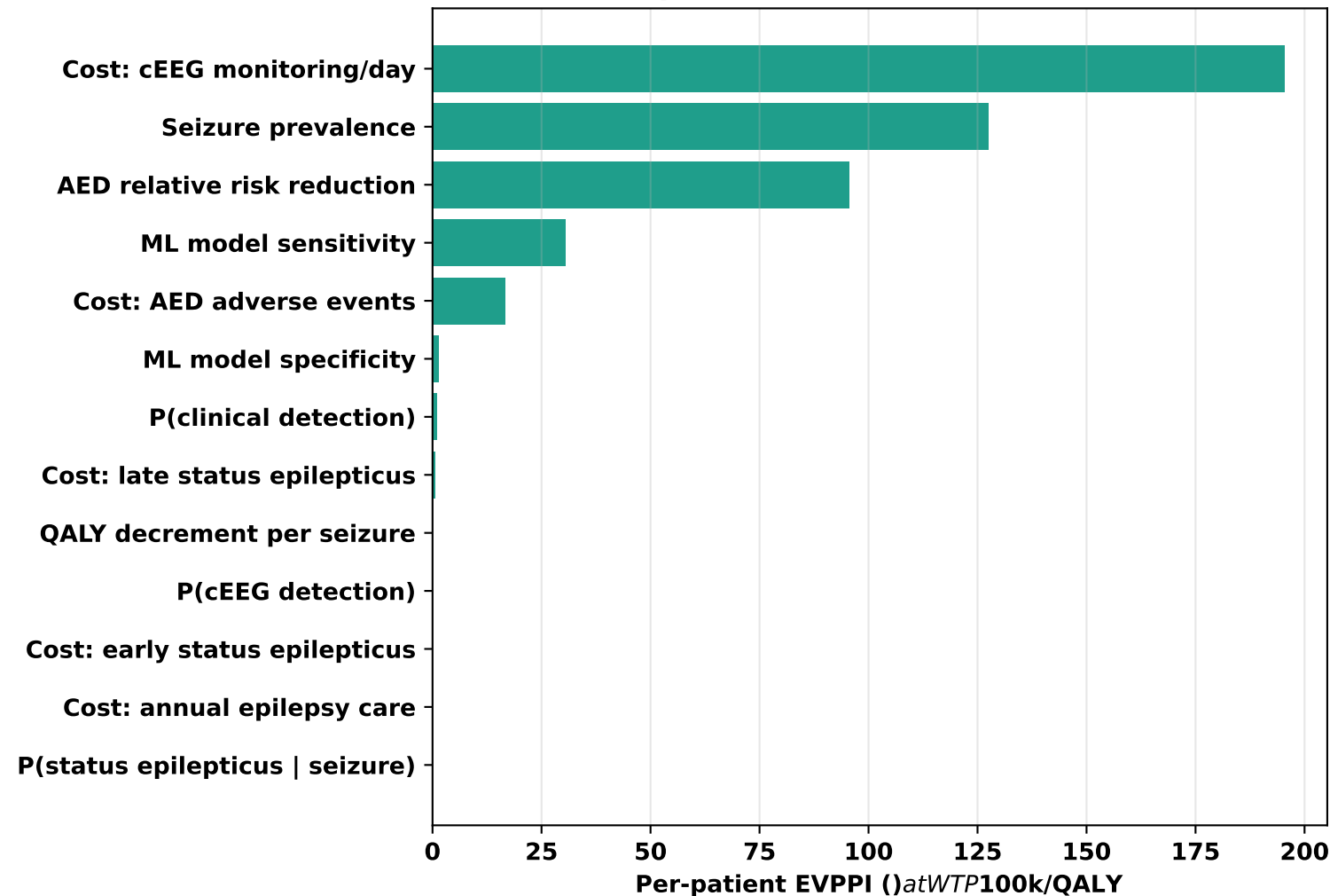
Per-parameter expected value of perfect information (EVPPI)
