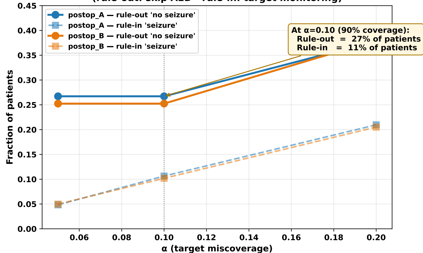
Clinical-utility — confident singleton predictions (rule-out: skip AED · rule-in: target monitoring)
