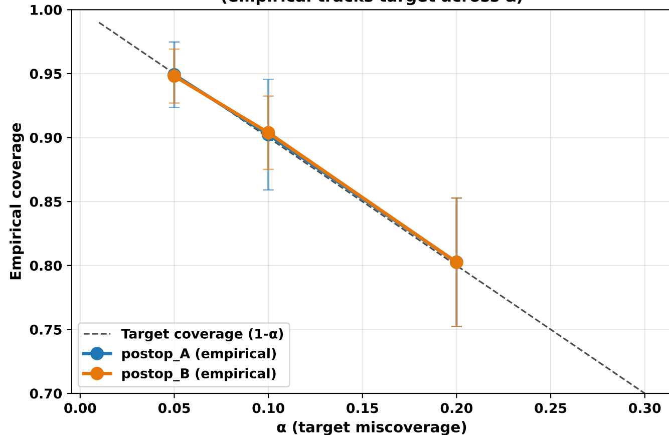
Coverage validation (empirical tracks target across \alpha )
