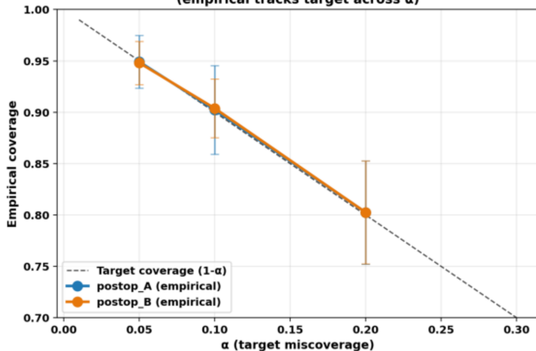
Coverage validation (empirical tracks target across \alpha )
