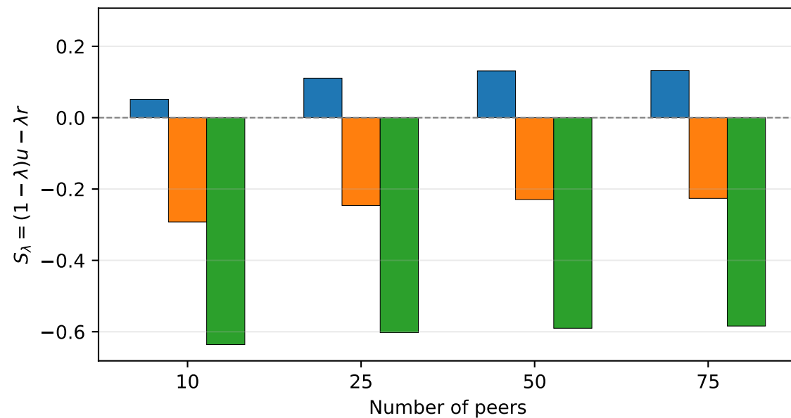
Topology-aware chunking
