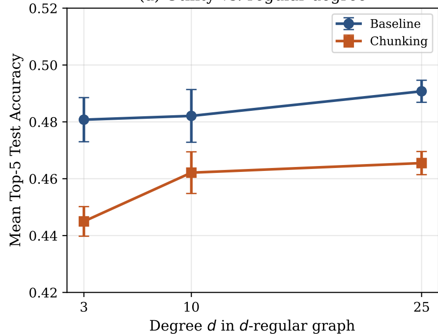
(a) Utility vs. regular degree
