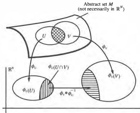
Figure 1: Manifold Charts
