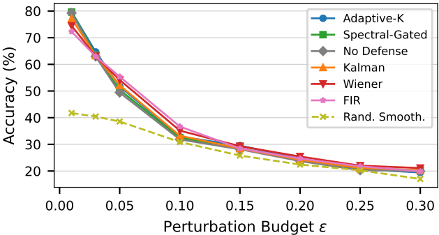
Accuracy vs. Budget — FGSM Attack
