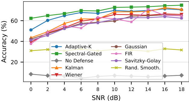
Accuracy vs. SNR — EAD-L1 Attack
