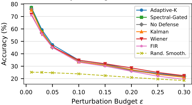
Accuracy vs. Budget — FGSM Attack
