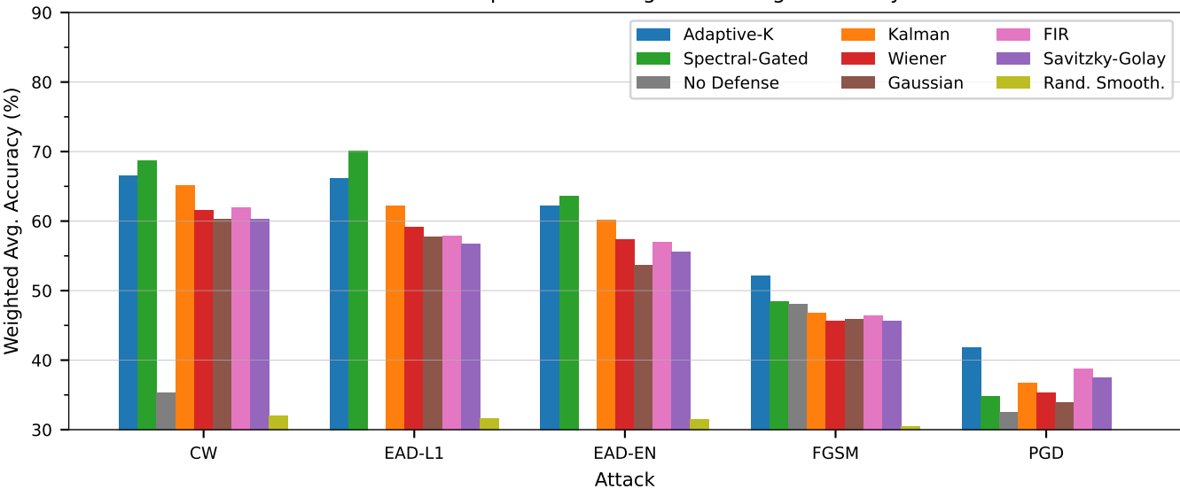
Defense Comparison — Weighted Average Accuracy
