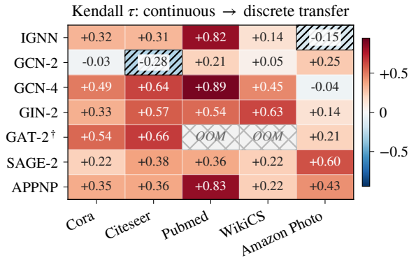
Fig. 7: Continuous-to-discrete transfer \tau across 7 architectures and 5 datasets (10 seeds, 330 runs). Cell values are mean Kendall \tau ; buckets: strong ( \tau > 0.5 ), moderate (0.3–0.5), weak (0–0.3), anti-correlated ( \tau < 0 , diagonal hatch); cross-hatch: GPU OOM. Deeper models (GCN-4, APPNP) and GAT † dominate.
