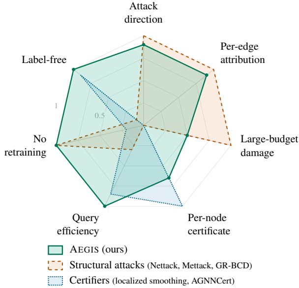
Figure 9: Method-positioning radar (qualitative levels; 0 at the centre, 1 at the outer ring; each polygon traces the frontier of its thread, i.e. the best any cited method achieves on that axis). Structural attacks (Zügner, Akbarnejad, and Günnemann 2018; Zügner and Günnemann 2019a; Geisler et al. 2021) own attack direction, per-edge ranking, and large-budget damage (the white-box gradient is the attribution oracle), but give no per-node certificate. Certifiers (Schuchardt et al. 2023; Li and Wang 2025) own the per-node certificate—AGNNCert is deterministic ( T=30\text{--}80 subgraph evaluations), localized smoothing is a collective certificate at \sim 10^5 samples/node—but name no vulnerability-driving edges and need specialised retraining. AEGIS reads attack direction, per-edge attribution, and a first-order per-node certificate off a single closed-form, label-free S_c query on an off-the-shelf model: it wins no specialist axis outright, but is the only method with nonzero mass on all seven. (AEGIS’s third capability, hardening via a \sigma_1(S_c) penalty, is evaluated separately in section 5.3.)
