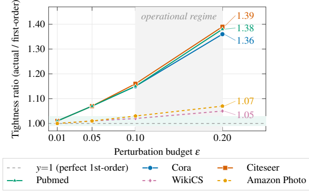
Figure 8: First-order tightness of the equilibrium-shift prediction versus the perturbation budget \varepsilon (full graph, mean over 10 seeds). The ratio is the true shift divided by the first-order prediction \sigma_1(S)\varepsilon ; it is 1 when the linearization is exact and rises as \varepsilon grows. Within the operational regime ( \varepsilon \leq 0.10 ) every curve stays below 1.16; only at \varepsilon = 0.20 do citation graphs (solid) reach 1.36–1.39, while product graphs (dashed) stay within 1.07. This shift-prediction ratio is distinct from the ranking tightness quoted elsewhere (1.00–1.02, Appendices F.5 and F.6), which is measured at the operational sub-graph scale; the figure traces the budget dependence that motivates capping \varepsilon in that regime.
