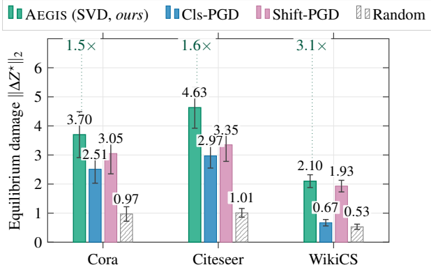
Figure 9: Equilibrium damage \|\Delta z^*\|_2 at \varepsilon=0.10 across 10 seeds, for the one-query AEGIS (SVD) attack against classification-loss PGD, IFT-gradient (shift) PGD, and a random baseline, on Cora, Citeseer, and WikiCS. Visual companion to table 3: one analytic AEGIS query inflicts 1.5–3.1 \times the damage of a 50-step Cls-PGD run per dataset, at a fraction of its cost.
