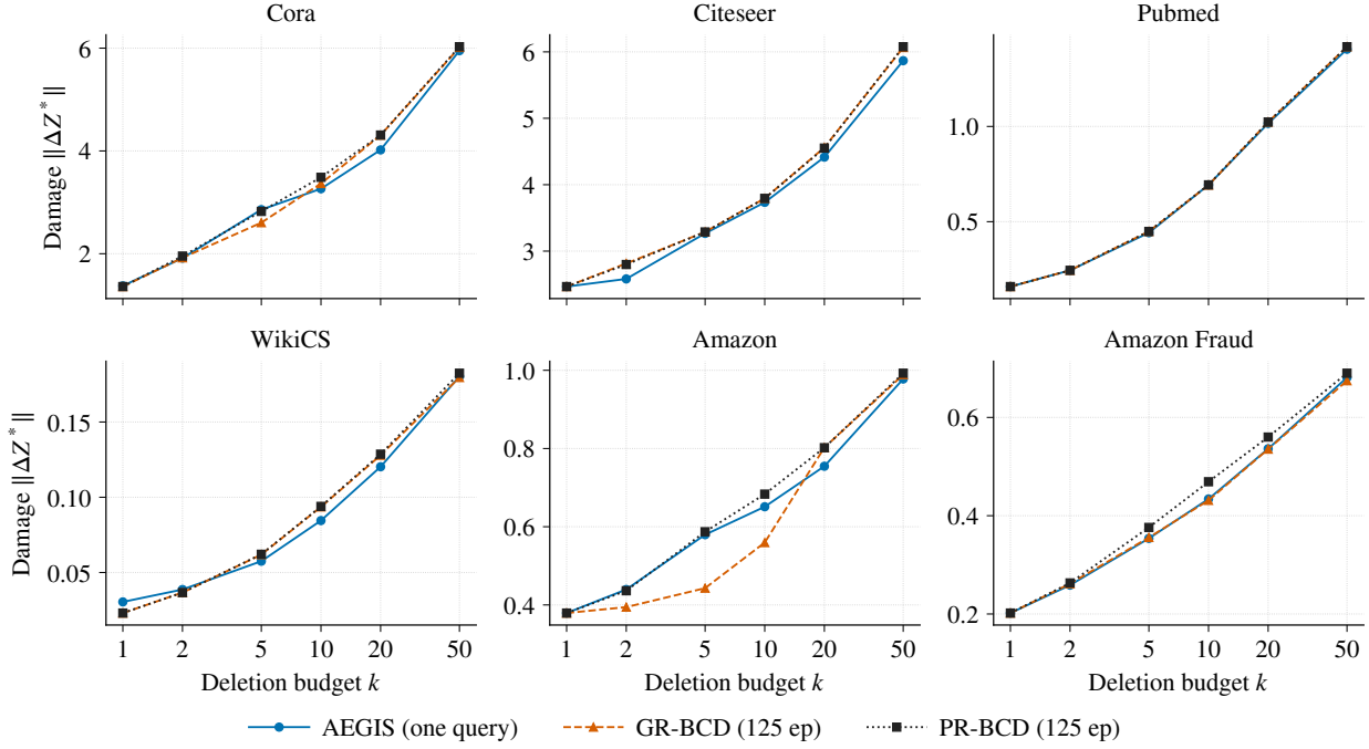
Figure 10: Damage-equivalence across the budget sweep (10 seeds). Absolute equilibrium-shift damage \|\Delta z^*\| of AEGIS’s single closed-form query against faithful 125-epoch GR-BCD and PR-BCD attackers (Geisler et al. 2021), per dataset, versus deletion budget k . AEGIS (blue) is an explicit curve; its near-coincidence with the two iterative attackers is the damage-equivalence: one label-free query recovers, and often exceeds, the equilibrium damage a 125-epoch optimizer reaches.
