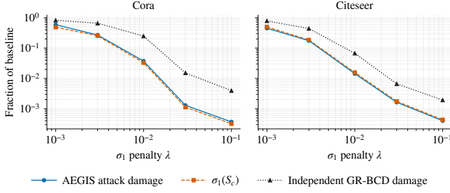
Figure 13: One knob, coherent movement: over the \sigma_1(S_c) penalty sweep, AEGIS attack damage, \sigma_1(S_c) , and an independent GR-BCD attacker’s damage fall together (fraction of the \lambda=0 baseline; 10 seeds).
