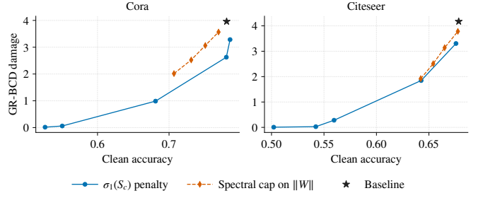
Figure 14: Independent-attacker frontier: at matched accuracy the \sigma_1(S_c) penalty blunts a faithful GR-BCD attacker more than a generic spectral cap on \|W\| (lower is better; 10 seeds).
