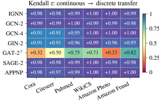
† GAT-2: 2-layer attention; finite-difference sensitivity (attention masks A ).
