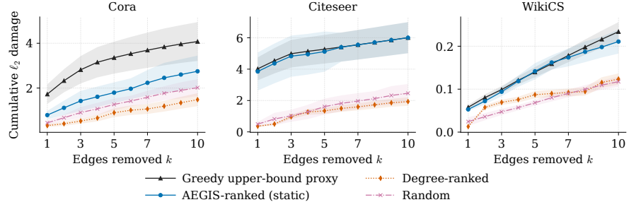
Figure 5: Cumulative damage from sequential discrete edge removal vs. k (IGNN, 50-node subgraph, 10 seeds). AEGIS matches label-aware Greedy on Citeseer/WikiCS and recovers 54–67% of its Cora damage at k=5-10 with no label access.
