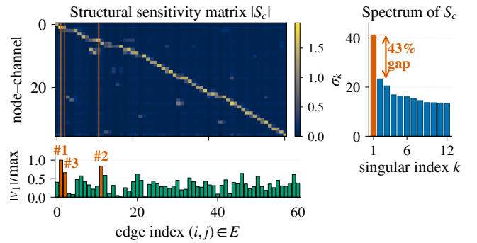
Figure 3: |S_c| on a 50-node Cora ego-graph (IGNN, N=50 , d=16 , |E|=61 , seed 0). Vermilion: top-3 edges by |v_1| (SVD-optimal direction). Sidebar: singular spectrum ( \sigma_1=41.2 , 43% gap to \sigma_2 ).
