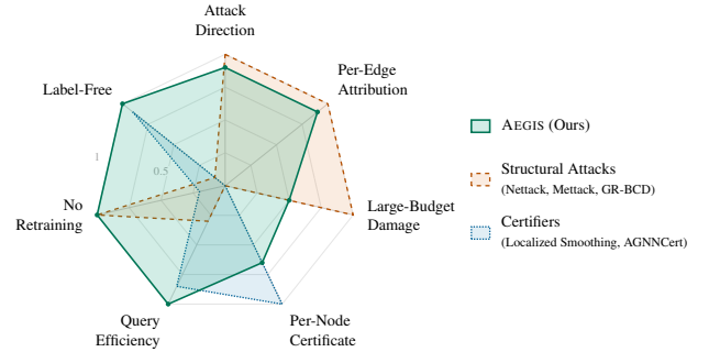
Figure 1: Seven-axis capability radar (frontier semantics; 0 at the centre, 1 at the rim): AEGIS wins no axis outright but is the only method that spans all seven from one object. Defense (the \sigma_1(S_c) penalty) is benchmarked separately (section 5.3); axis definitions and per-method scoring are in appendix F.2.
