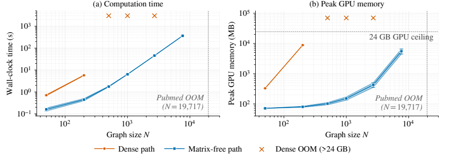
Figure 12: Dense vs. matrix-free AEGIS pipeline (RTX 4090). The dense path scales as O((Nd)^3) , exceeding 24 GB beyond N=200 ; the matrix-free path is roughly O(N \log N) in time and sub-linear in memory, reaching Amazon Photo ( N=7,650 ) at 365 s and 5.5 GB.
